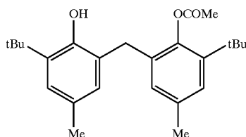
Stabilizer St-1
