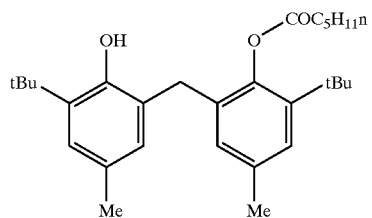
Stabilizer St-2
