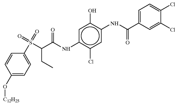
Coupler CC-1
