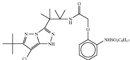
Coupler MC-1
