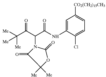
Coupler YC-1
