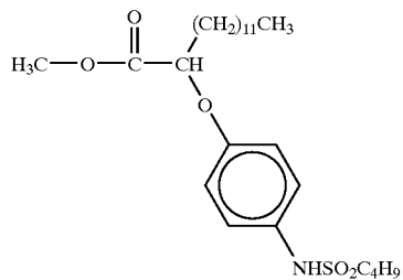
Stabilizer St-3
