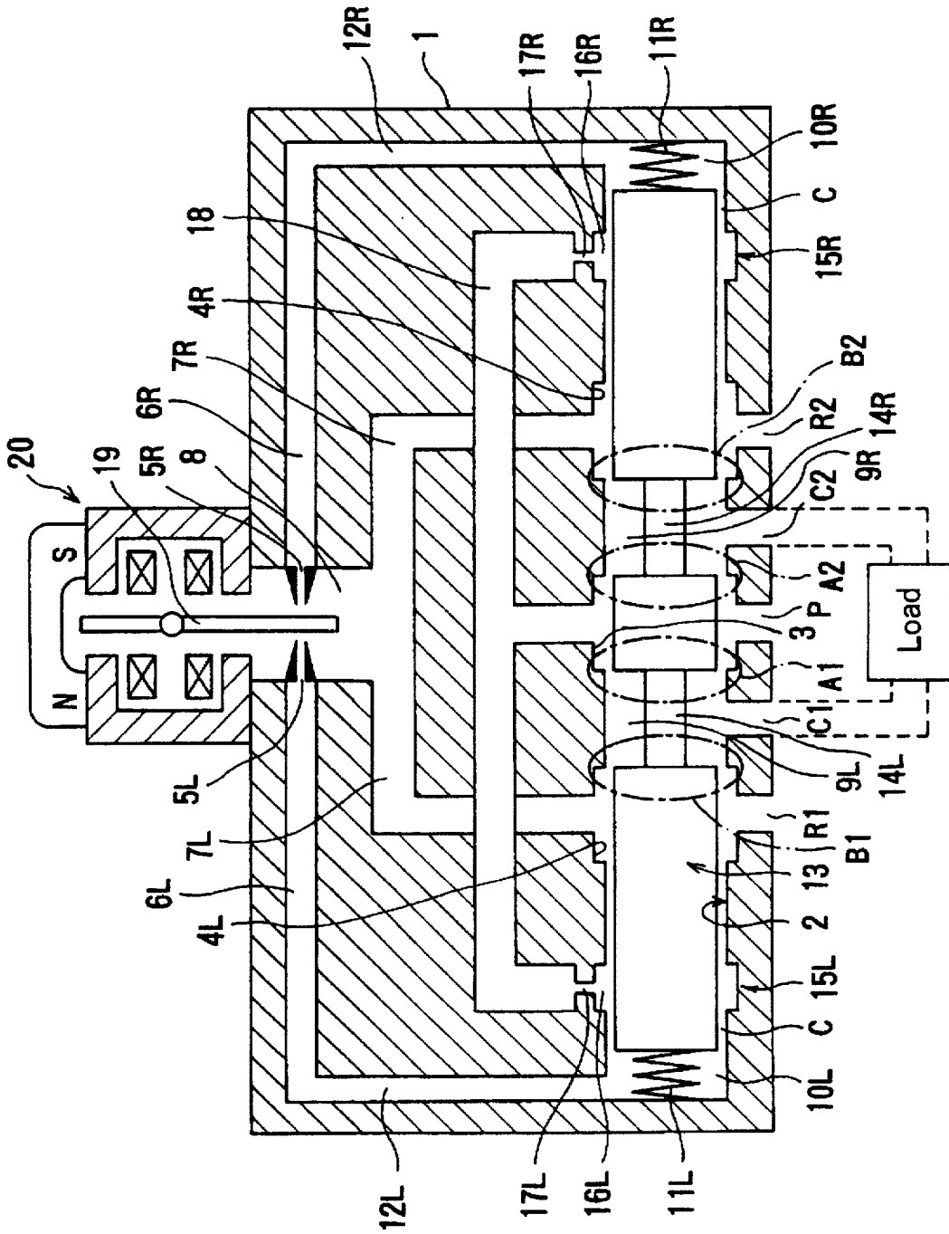
FIG. 10 RELATED ART
