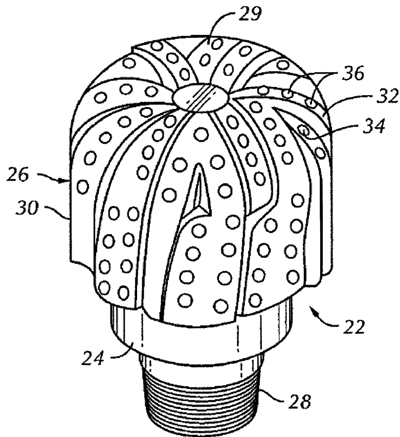
FIG. 2 (Prior Art)
