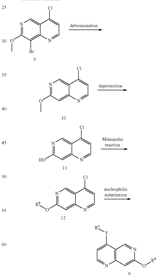
Reaction Scheme 2:
