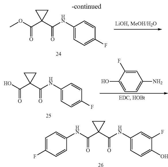
1-(methoxycarbonyl) Cyclopropane Monocarboxylic Acid (23)
