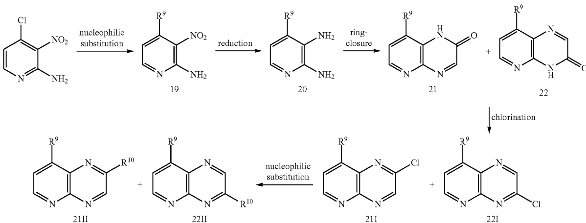
Reaction scheme 5:
