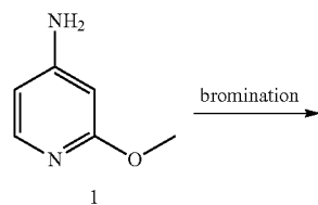
Reaction scheme 1:
