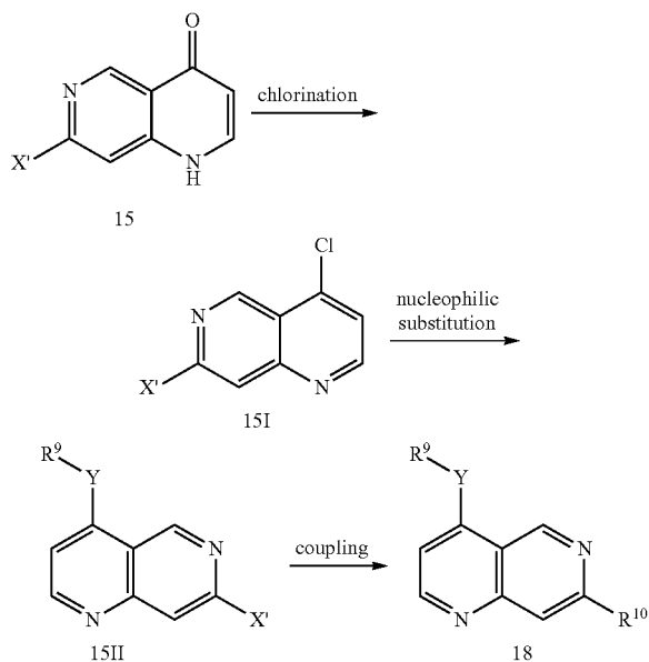
Reaction scheme 4:
