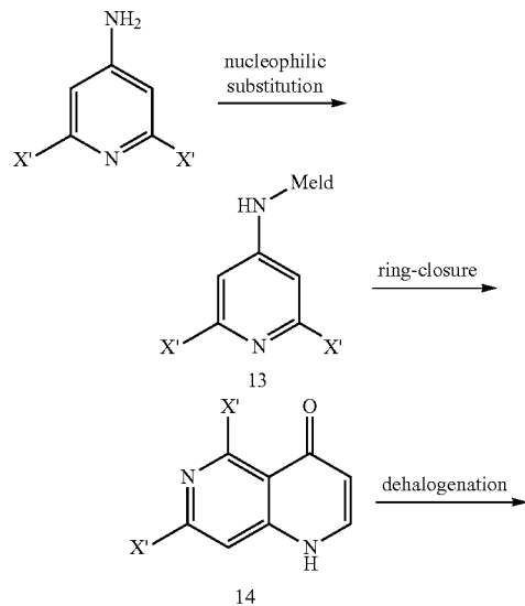
Reaction scheme 3:
