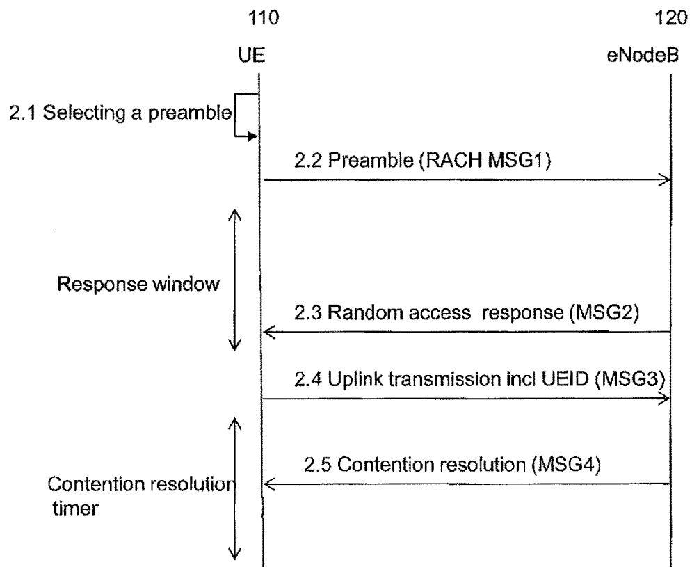
Fig. 2 (prior art)
