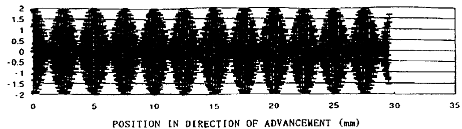
(b) COMPOSITE WAVE OF CHARGING BIAS AND DEVELOPING BIAS (SAME PHASE START)
