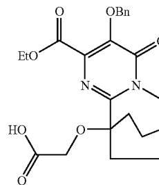
Intermediate 141
