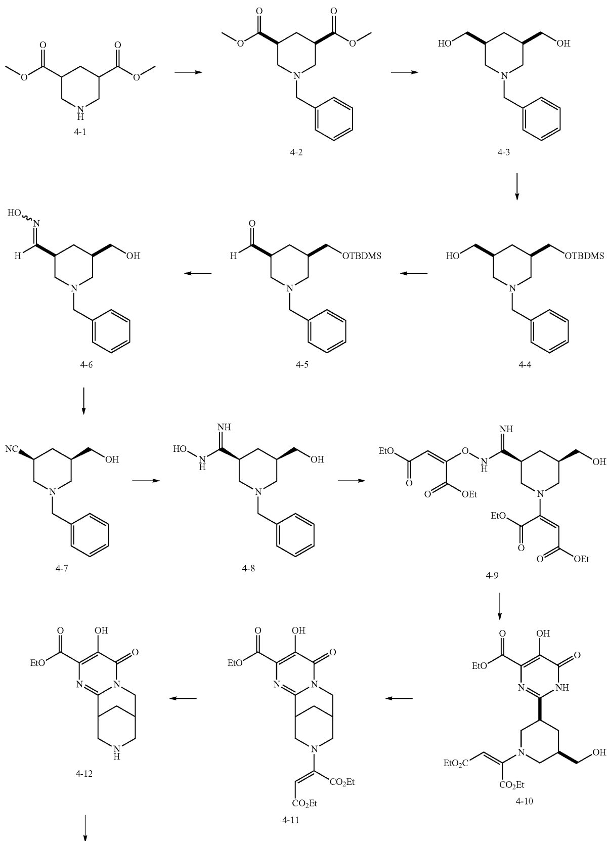
Scheme IV
