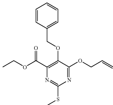
Intermediate 144
