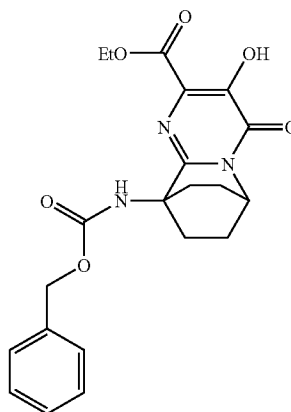
Intermediate 59
