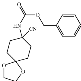
Intermediate 53
