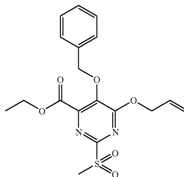
Intermediate 145
