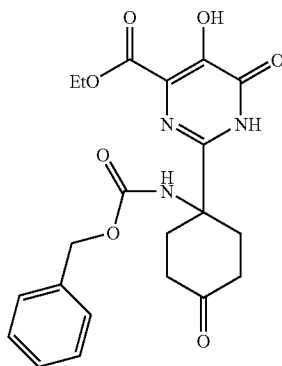
Intermediate 56
