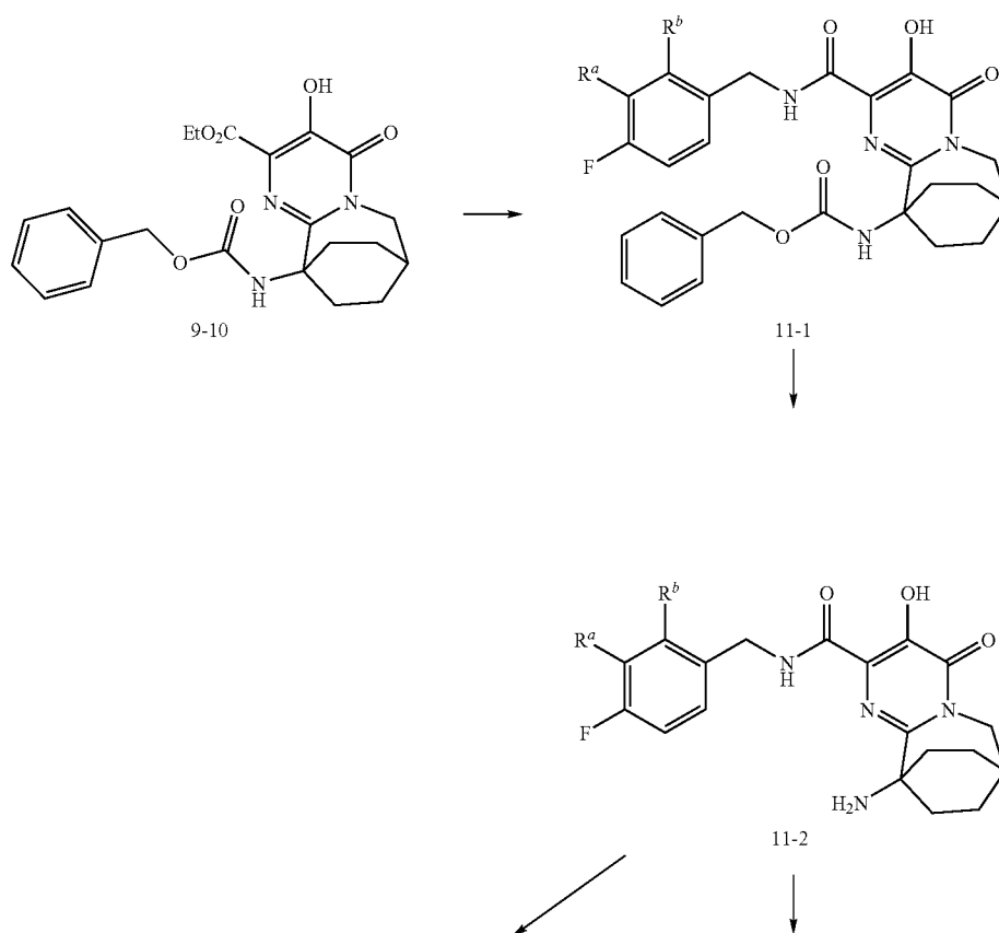
Scheme XI
