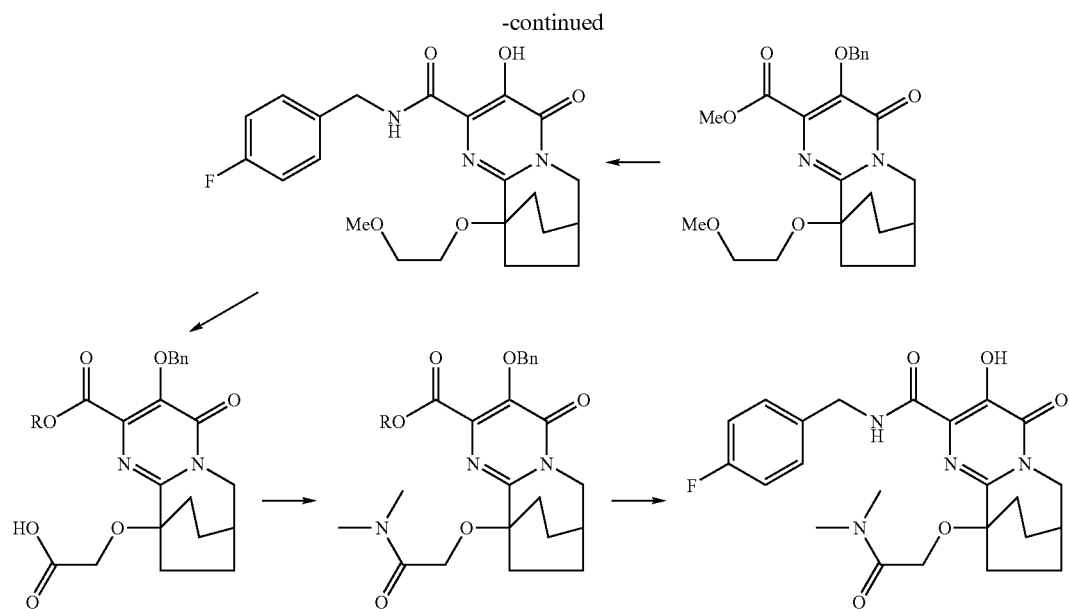
Scheme XXXIV
