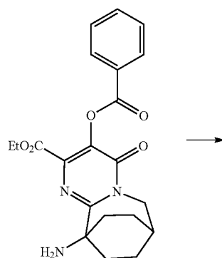
Scheme XX
