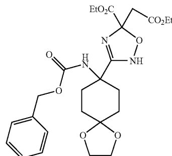
Intermediate 54
