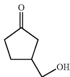
Intermediate 104
