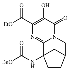
Intermediate 105
