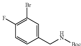
Intermediate 19
