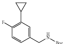
Intermediate 20
