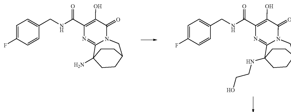
Scheme XXI
