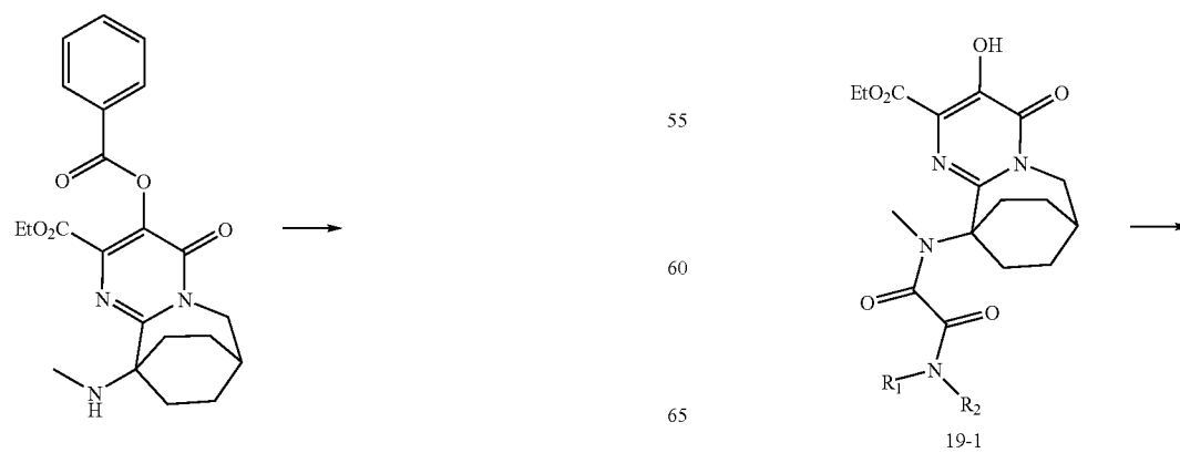
Scheme XIX
