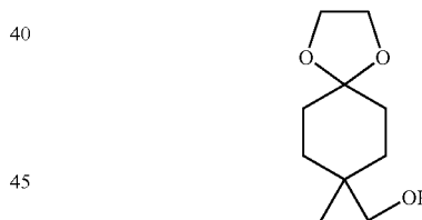
Intermediate 83
