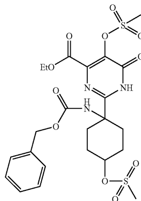
Intermediate 58
