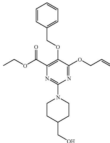
Intermediate 146
