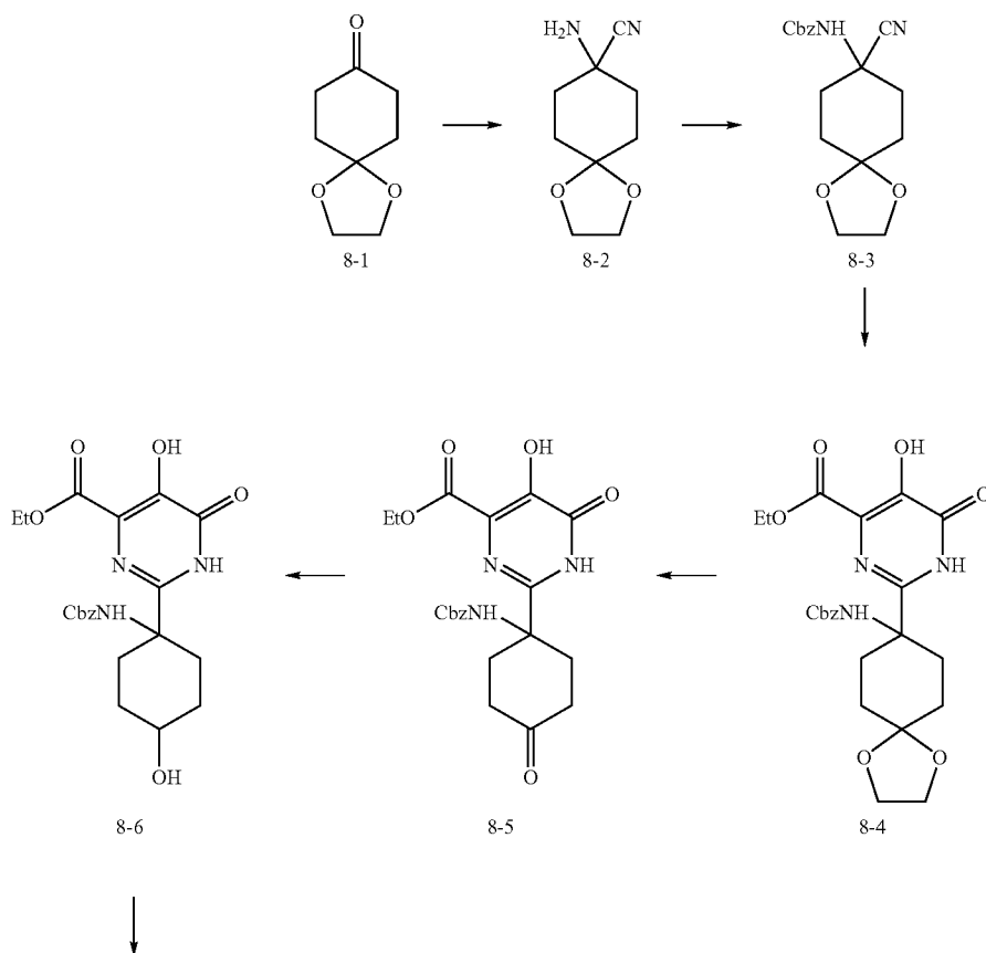
Scheme VIII
