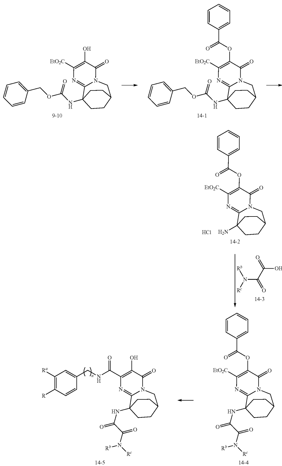
Scheme XIV
