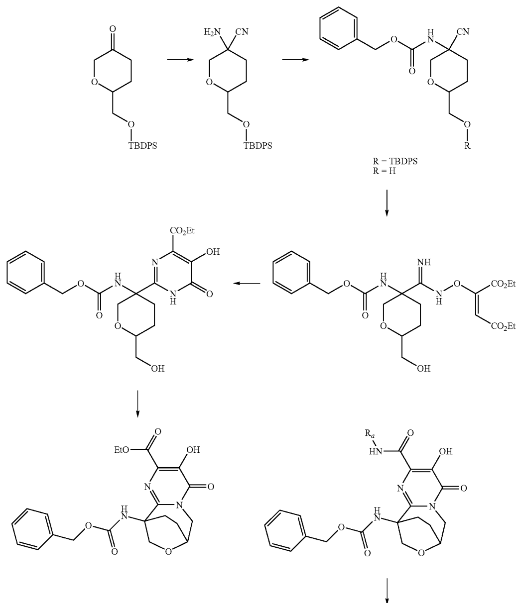
Scheme XXXI
