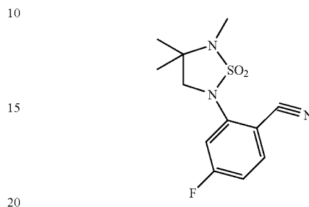
Intermediate 13
