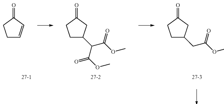
Scheme XXVII
