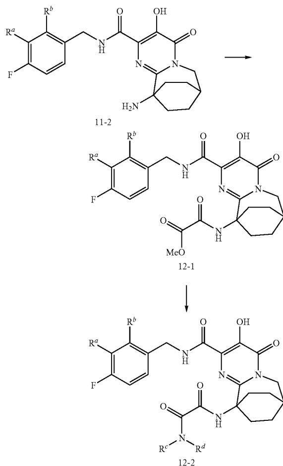
Scheme XII
