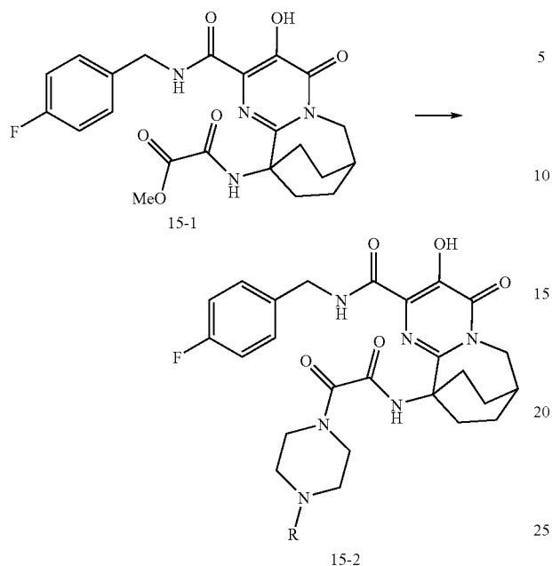
Scheme XV
