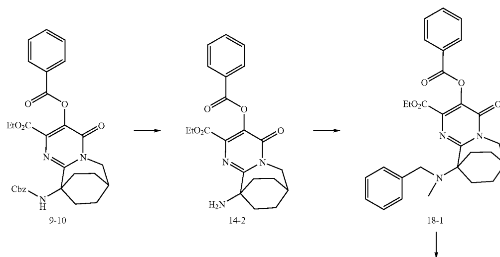
Scheme XVIII
