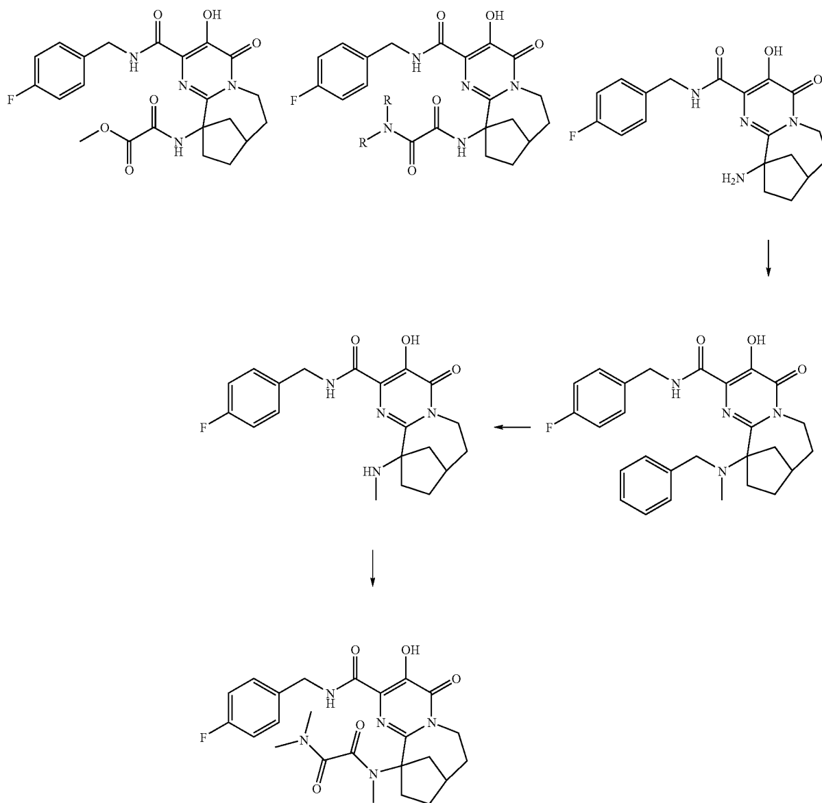
Scheme XXIX
