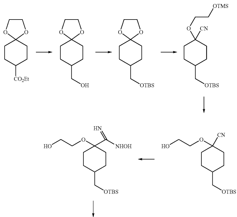
Scheme XXXII
