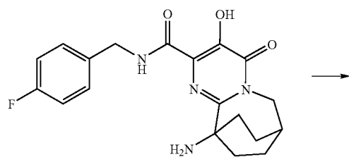
Scheme XXII
