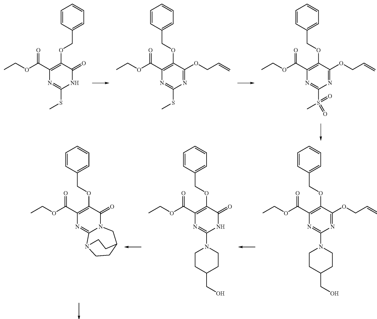
Scheme XXXIV
