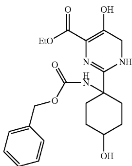
Intermediate 57
