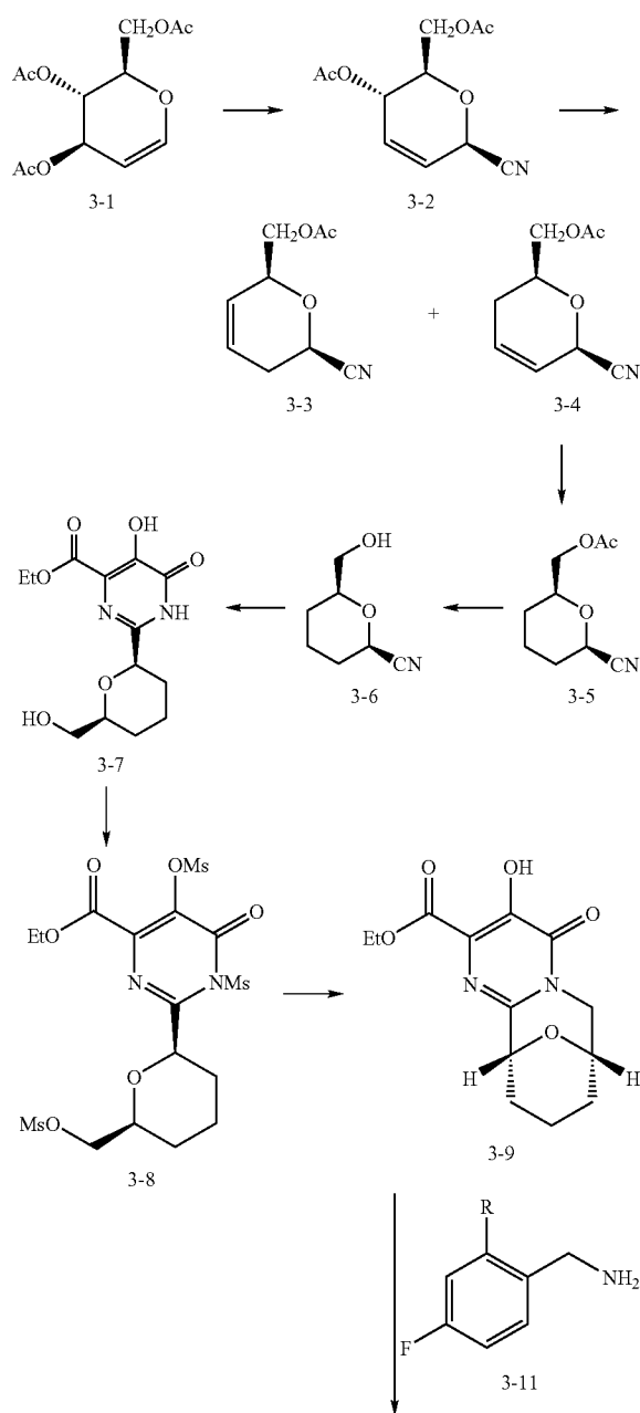
Scheme III
