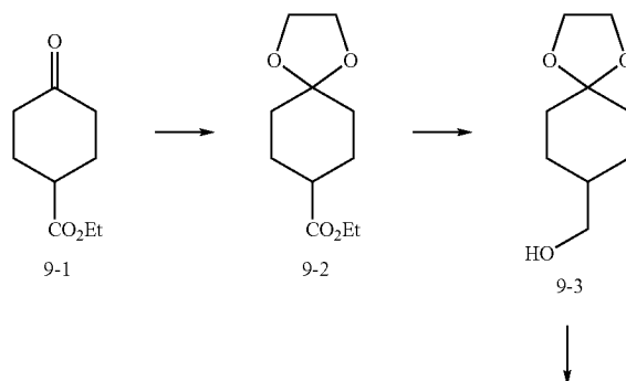
Scheme IX
