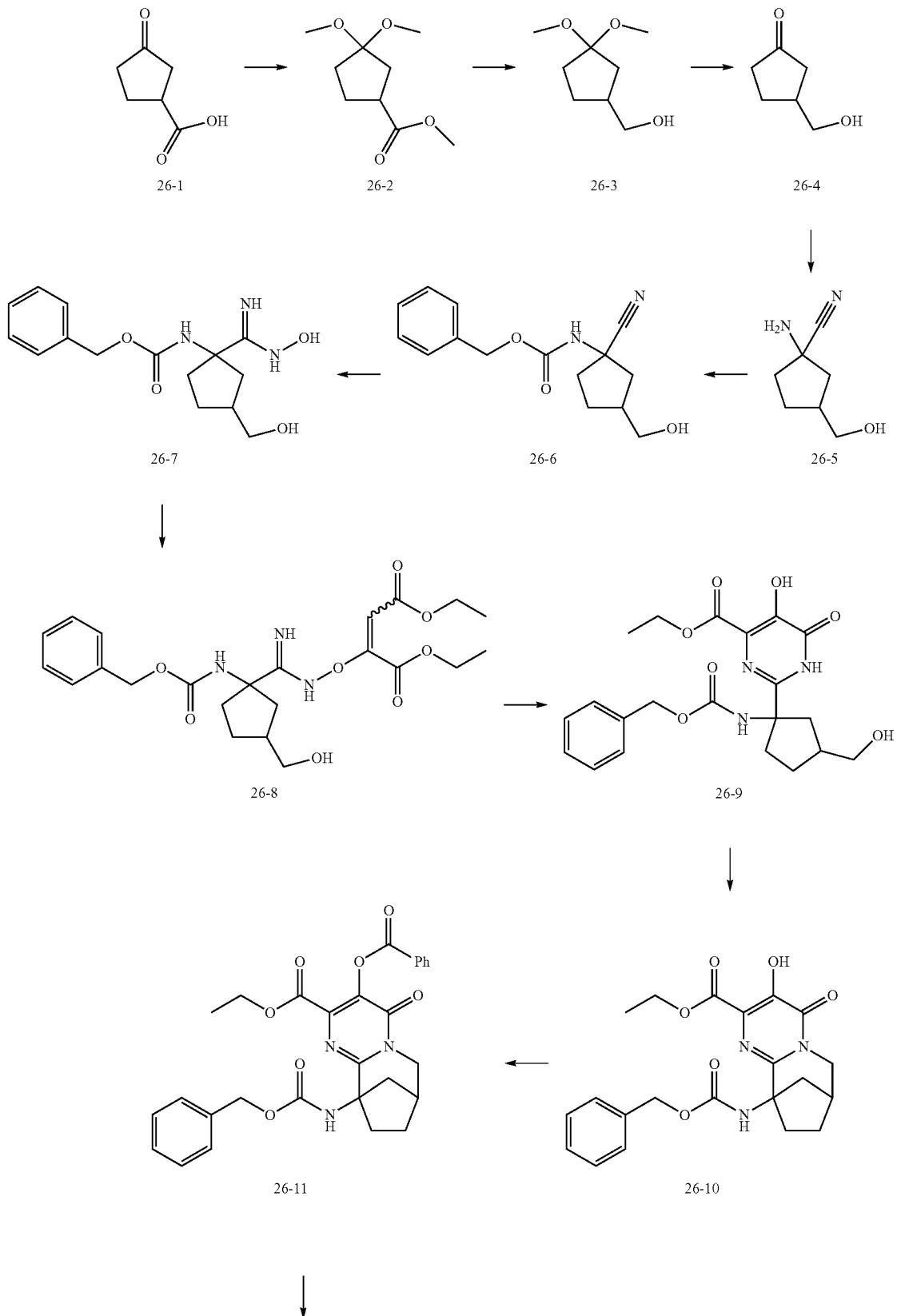
Scheme XXVI
