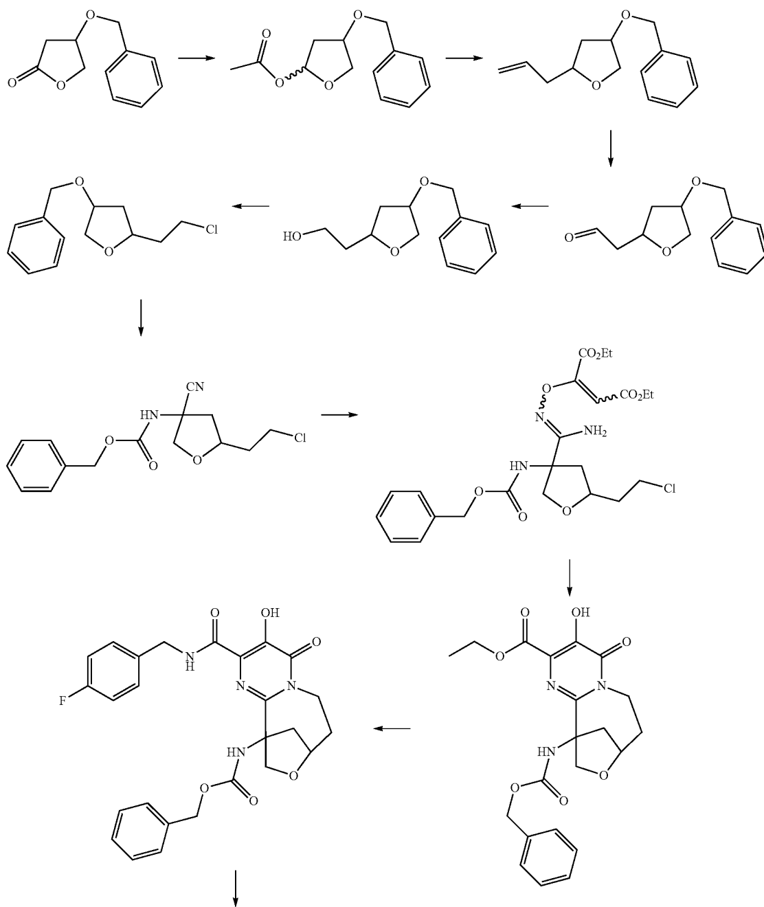
Scheme XXX
