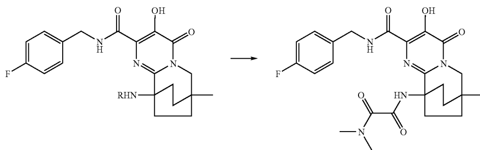
Scheme XXIV
