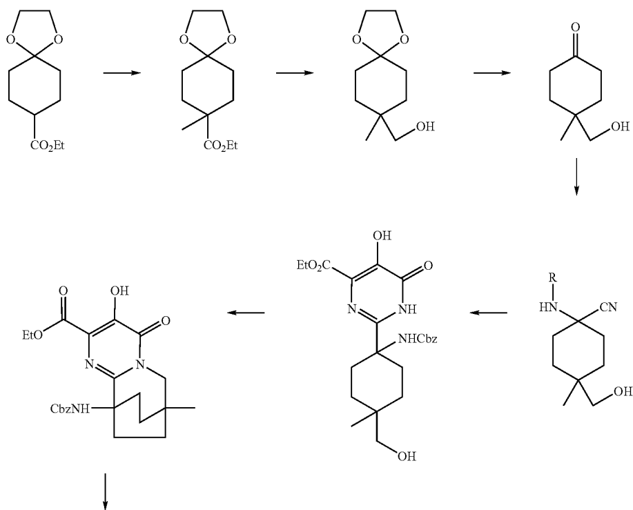
Scheme XXIII
