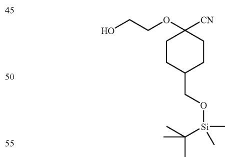
Intermediate 133
