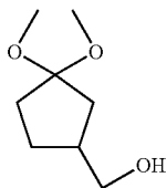
Intermediate 103
