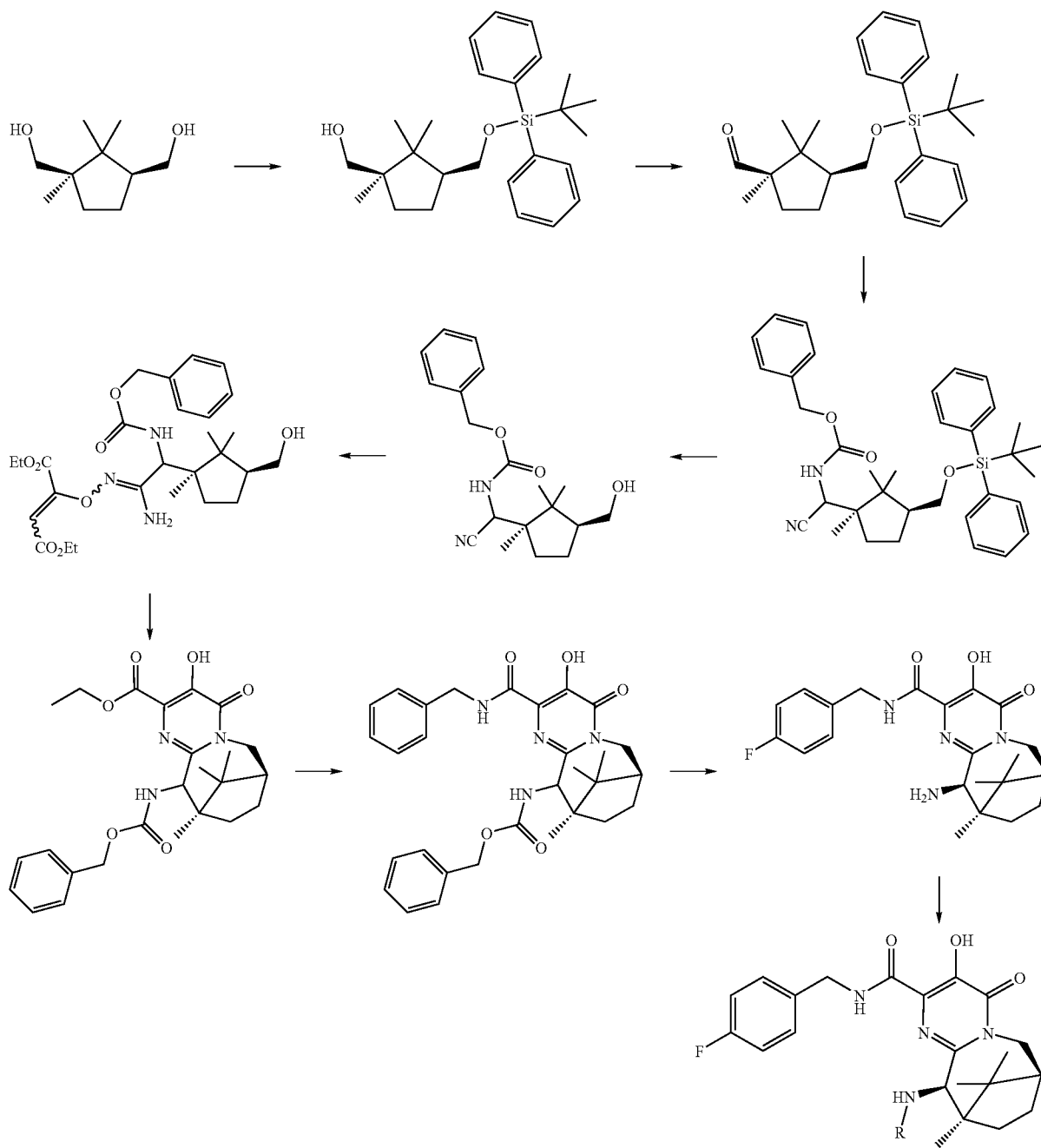
Scheme XXIV
