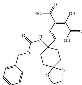
Intermediate 55
