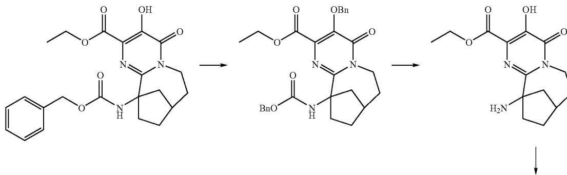
Scheme XXIX
