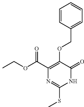
Intermediate 143
