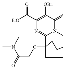
Intermediate 142
