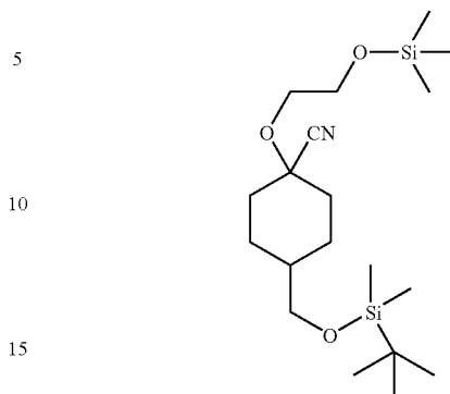
Intermediate 132
