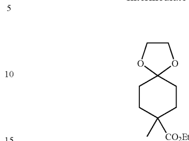
Intermediate 82
