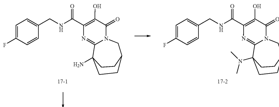
Scheme XVII
