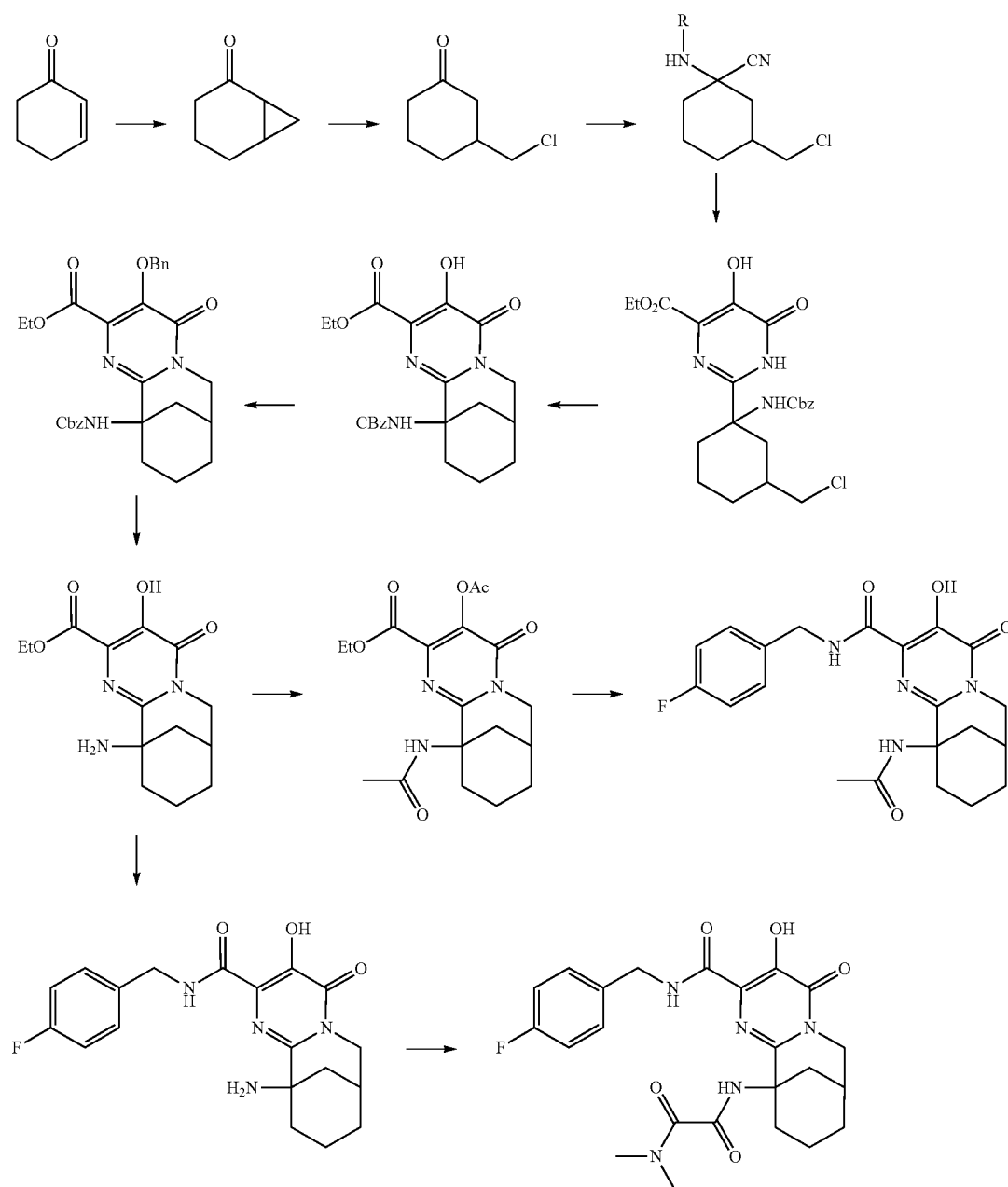
Scheme XXV
