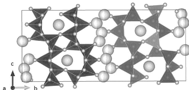
Crystal structure of Sr_3Si_8O_4N_{10}
