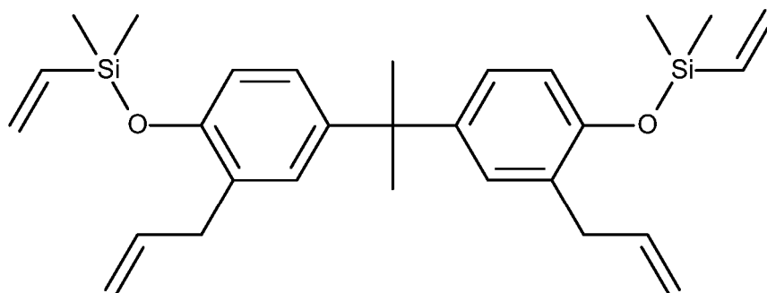
([2-allyl-4-[1-[3-allyl-4-[dimethyl(vinyl)silyl]oxy-phenyl]-1-methyl-ethyl]phenoxy]-dimethyl-vinylsilane).
