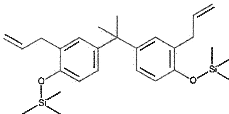
(([2-Allyl-4-[1-(3-allyl-4-trimethoxysiloxyphenyl)-1-methylethyl]phenoxy]-trimethylsilan))
