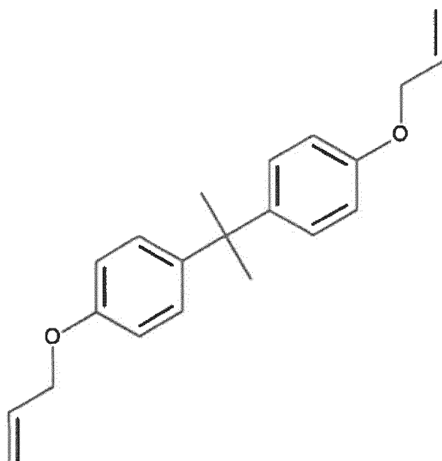
(1-Allyloxy-4-[1-(4-allyloxyphenyl)-1-methylethyl]benzol (Bisphenol A-Diallylether)))
