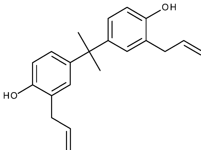
(2-allyl-4-[1-(3-allyl-4-hydroxy-phenyl)-1-methyl-ethyl]phenol (2,2'-diallyl bisphenol A))
