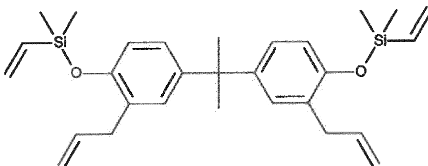
(([2-Allyl-4-[1-[3-allyl-4-[dimethyl(vinylsilyl)oxyphenyl]-1-methylethyl]phenoxy]-dimethylvinylsilan).
