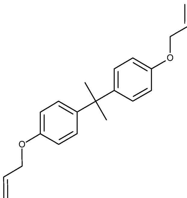
(1-allyloxy-4-[1-(4-allyloxyphenyl)-1-methyl-ethyl]benzene (bisphenol A diallyl ether))
