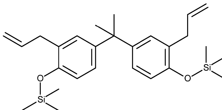
([2-allyl-4-[1-(3-allyl-4-trimethylsilyloxy-phenyl)-1-methyl-ethyl]phenoxy]-trimethyl-silane)),
