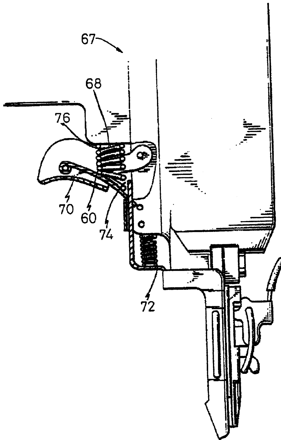
Fig. 12 PRIOR ART
