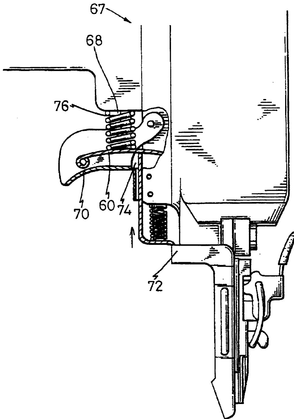
Fig. 9 PRIOR ART
