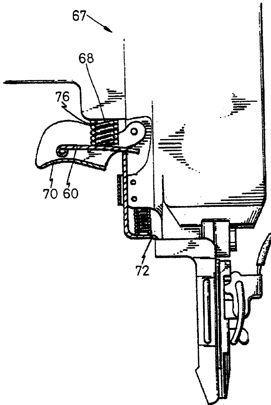
Fig. 10 PRIOR ART
