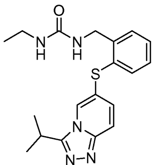
Y1X (1-ethyl-3-(2-([3-(1-methylethyl)[1,2,4]triazolo[4,3-a]pyridine-6-yl]sulfanyl)benzyl)urea
