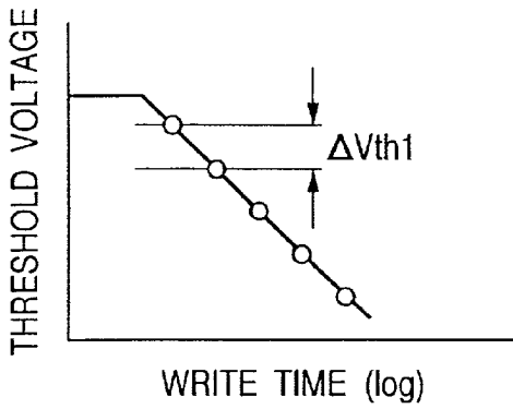
WRITE CHARACTERISTIC
