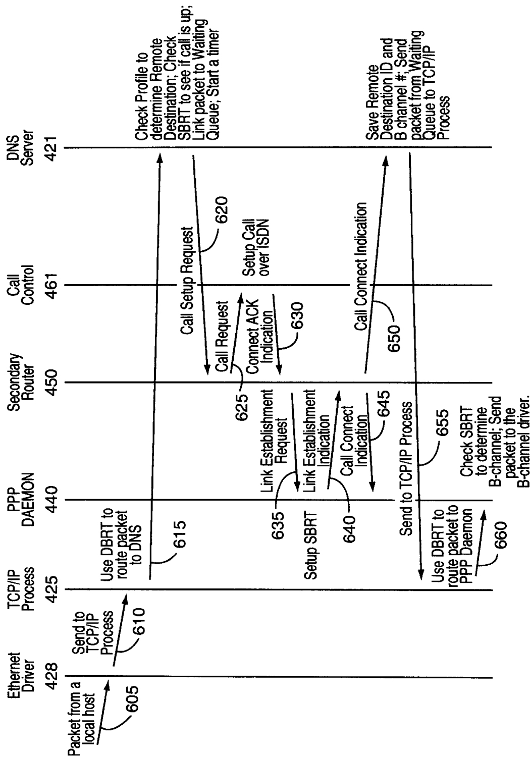
FIG. 6 ISDN CALL SETUP DUE TO DNS REQUEST
