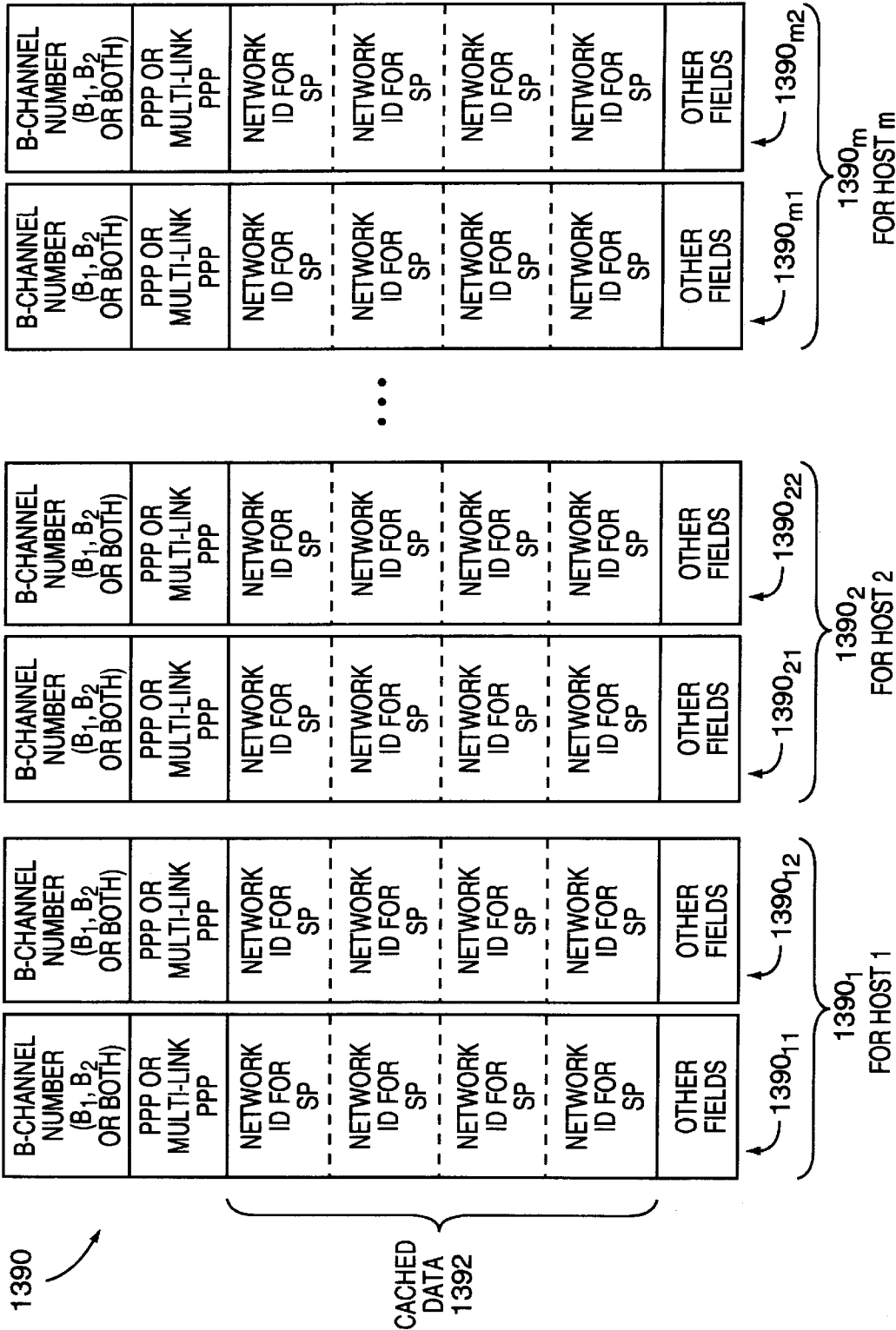
FIG. 13D SOURCE-BASED ROUTING TABLE 446
