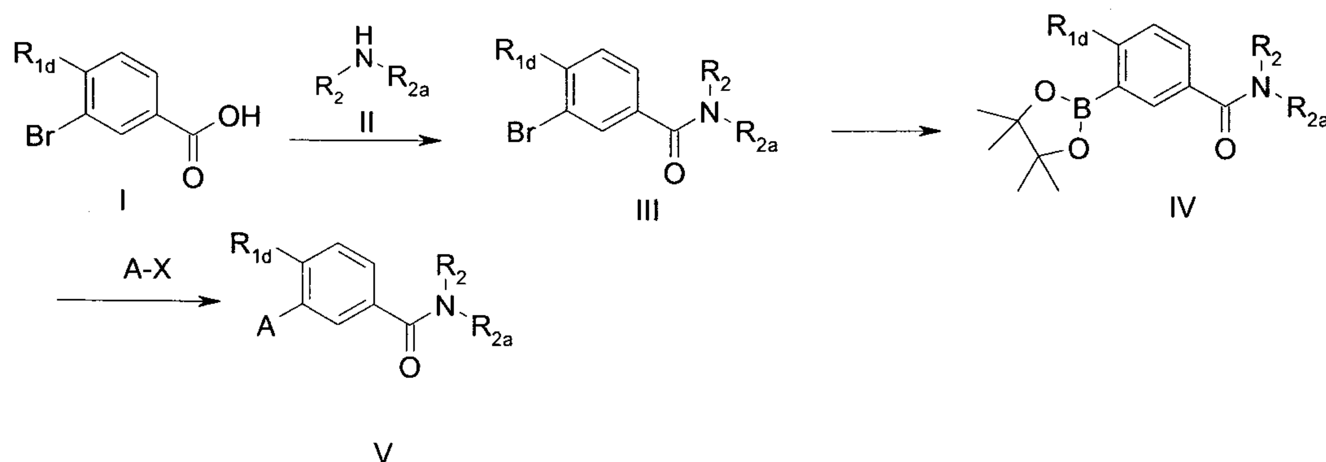
Scheme 1
