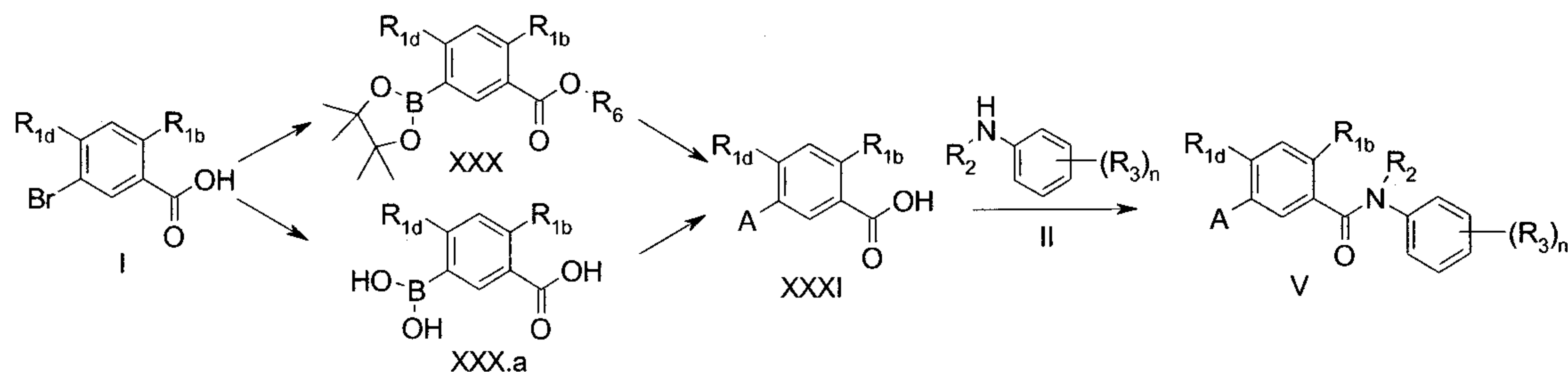
Scheme 11
