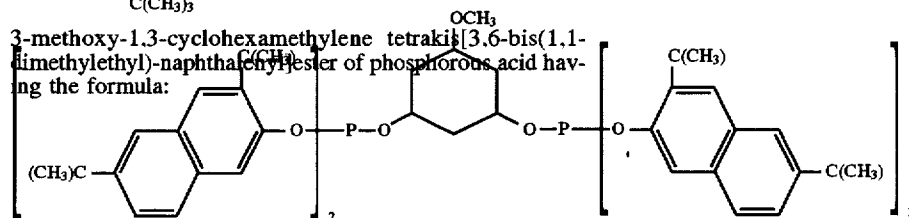
Ligand S
