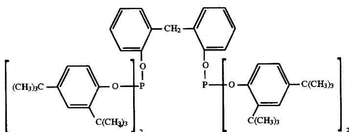
Ligand U
