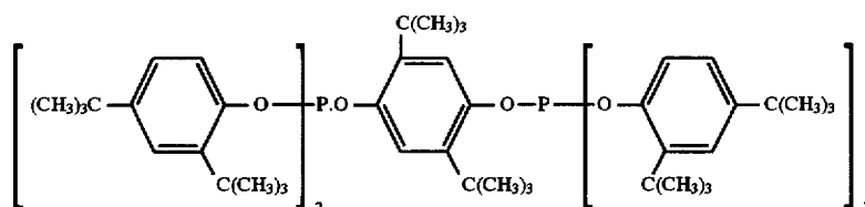
Ligand R
