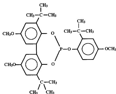
Ligand A
