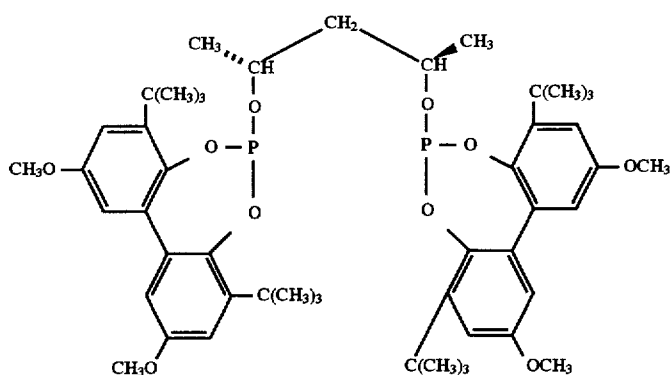
Ligand M
