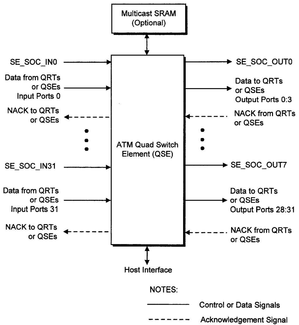
QSE Interface Block Diagram
