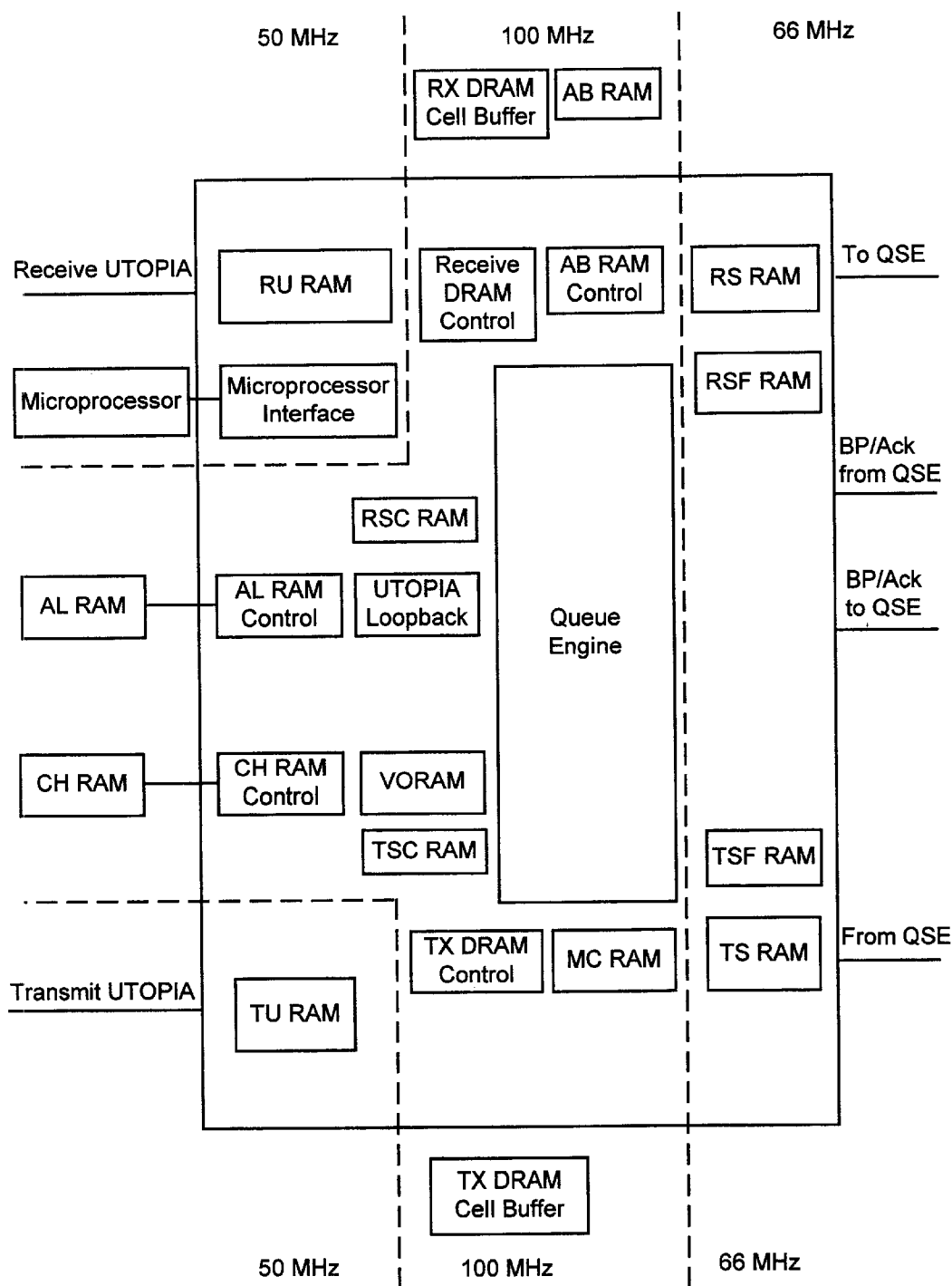
System Diagram of Internal QRT Blocks and External RAM FIG. 7
