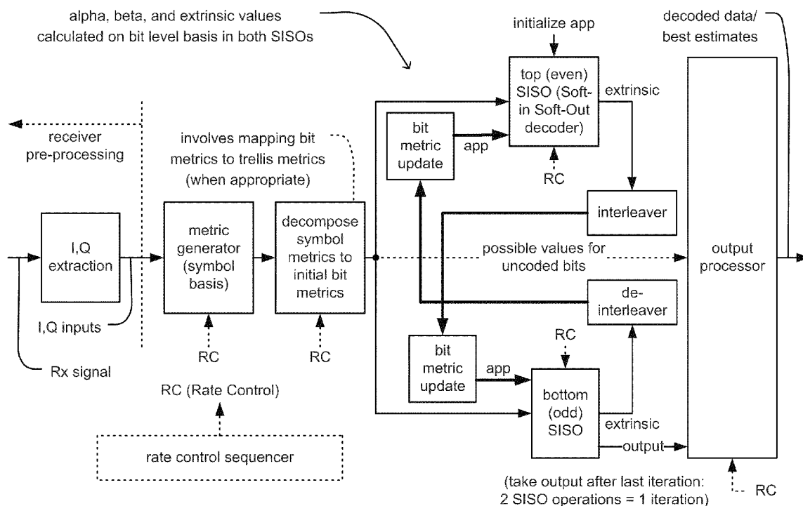
TTCM (Turbo Trellis Coded Modulation) decoder system
