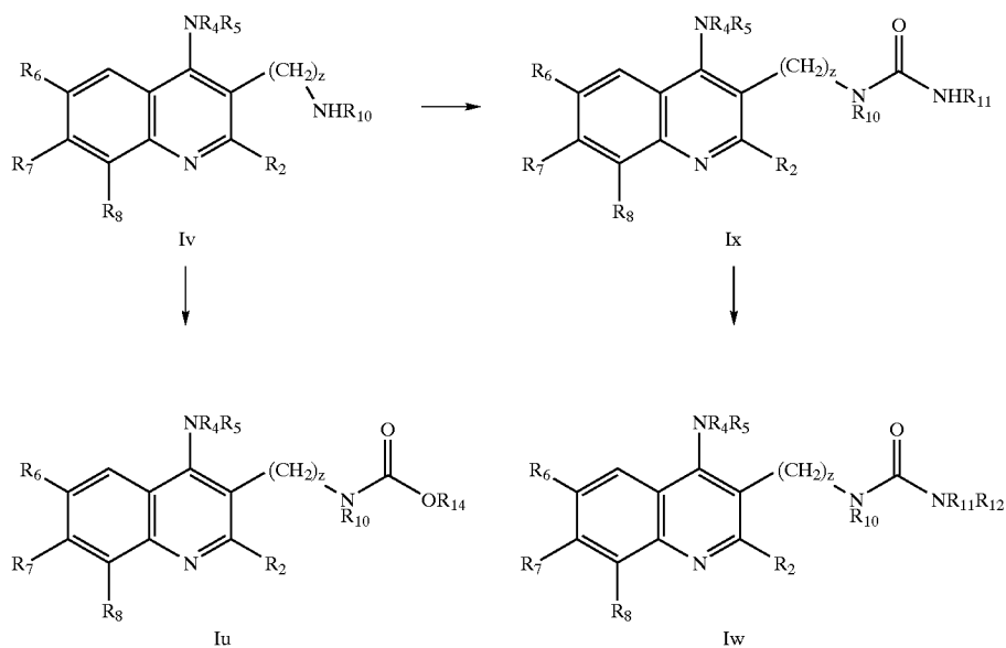
SCHEME VII
