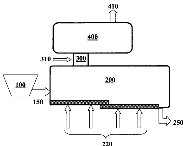
FIG. 1: Schematic Diagram of One Embodiment of Gasification Process: 2-Stage Gasification Process.
