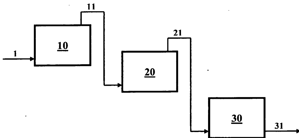
FIG 2: Schematic Diagram of Process to Produce Ethanol via Gasification of Carbonaceous Material.
