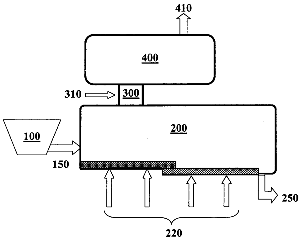
FIG. 1: Schematic Diagram of One Embodiment of Gasification Process: 2-Stage Gasification Process.
