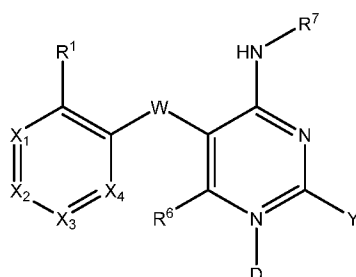
Formula 1m.
