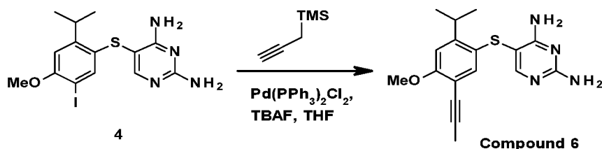
Scheme J
