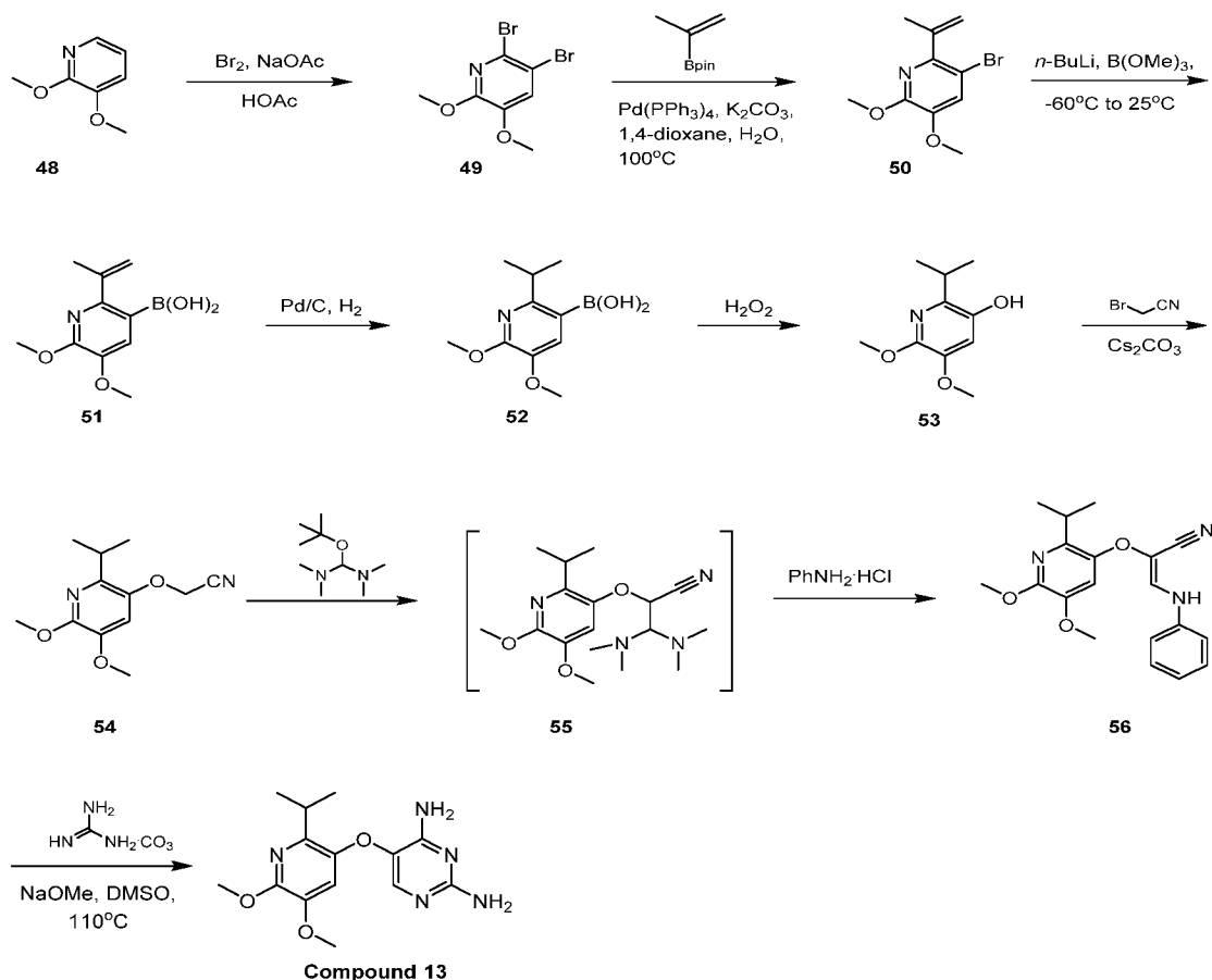
Scheme S
