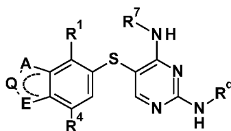
Formula 5
