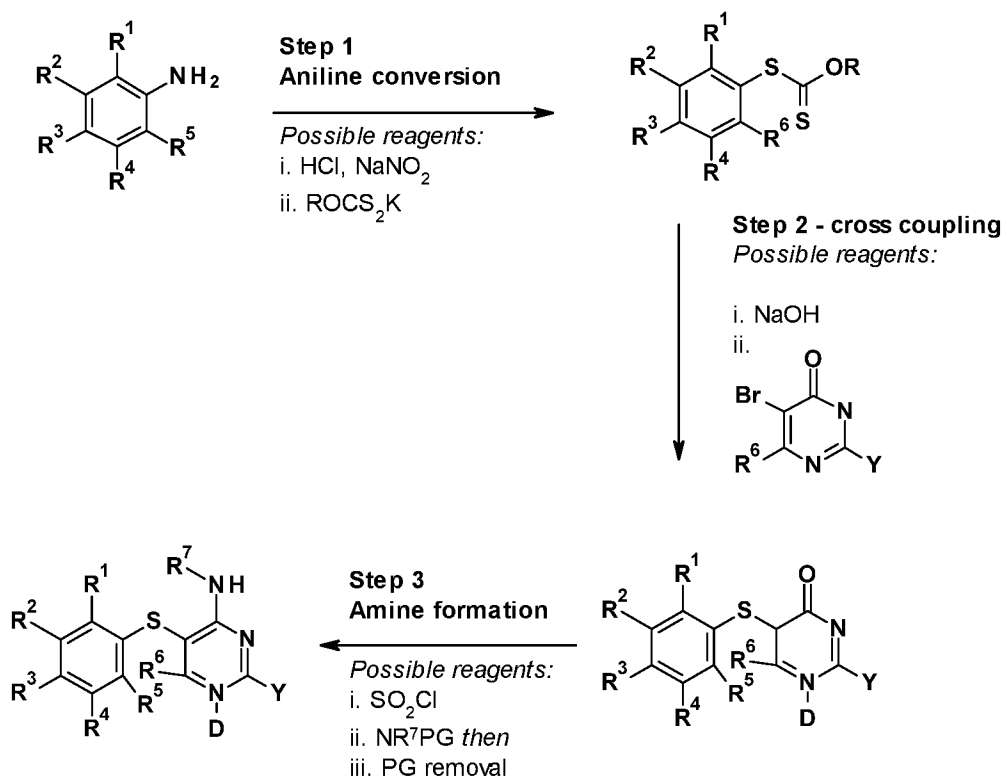
Scheme A
