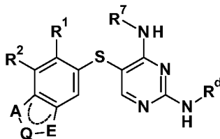
Formula 4
