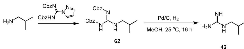
Scheme 20
