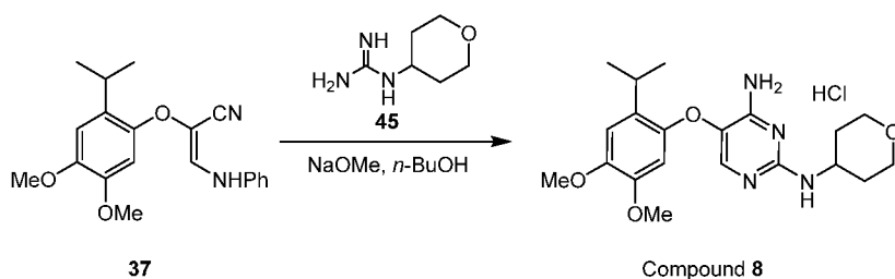
Scheme 11
