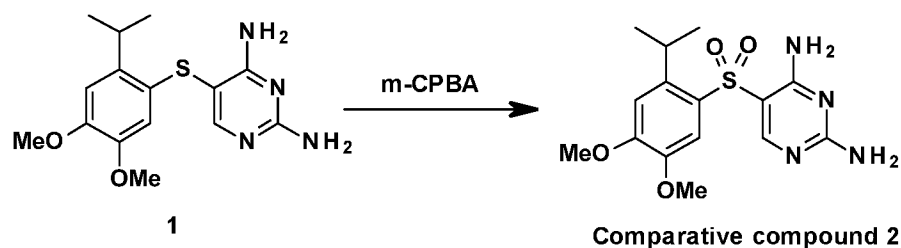
Scheme R
