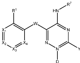
Formula 1l.
