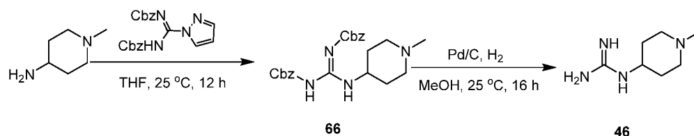
Scheme 24
