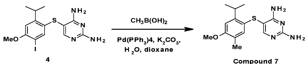
Scheme K
