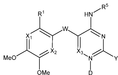
Formula 1n
