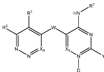
Formula 1f
