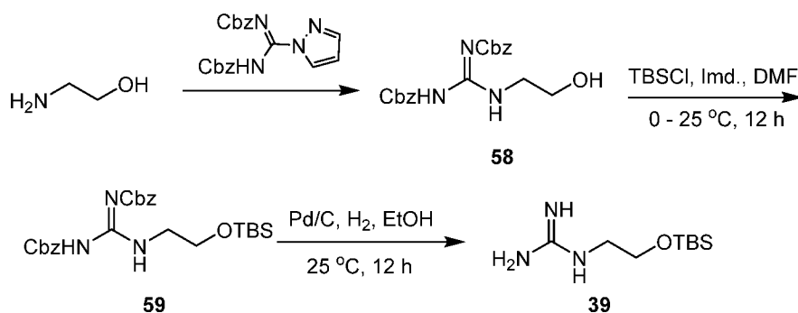
Scheme 17
