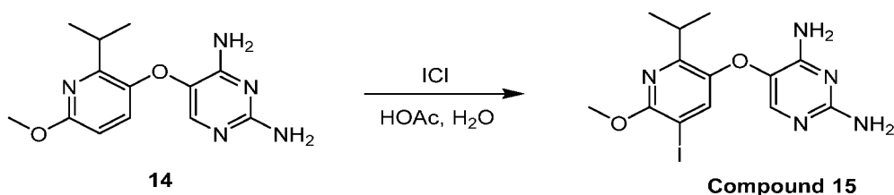
Scheme U
