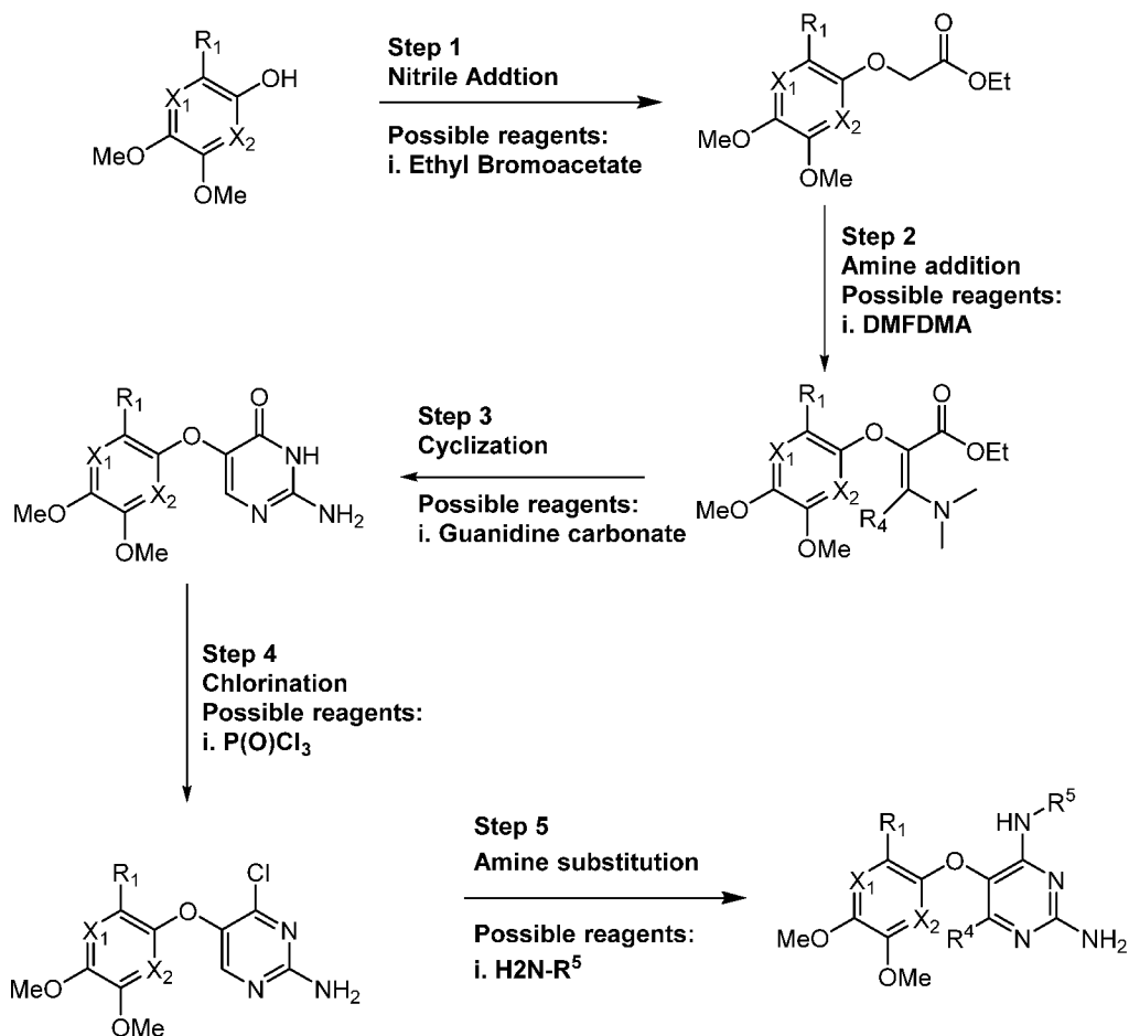
Scheme 3
