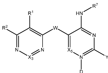
Formula 1g.
