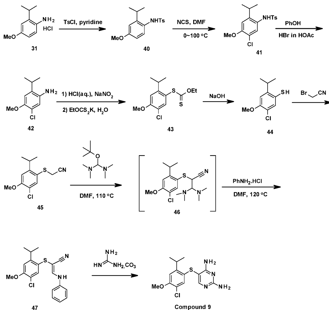
Scheme M
