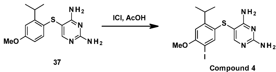
Scheme H
