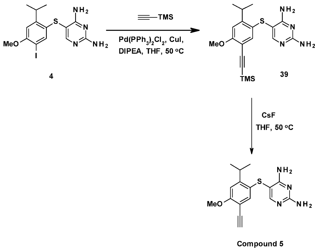
Scheme I
