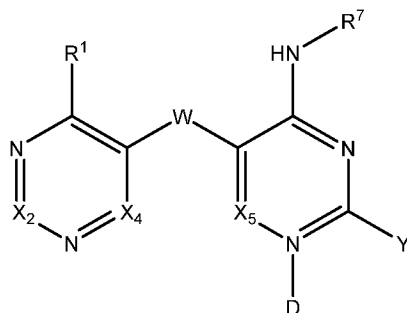
Formula 1j.
