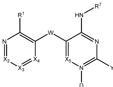
Formula 1b.
