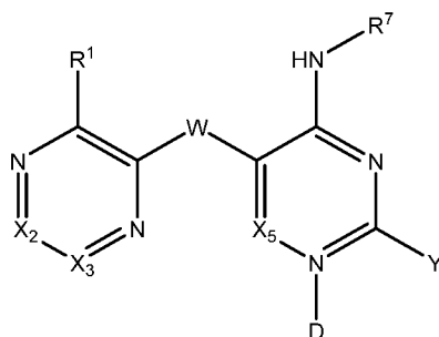
Formula 1k.
