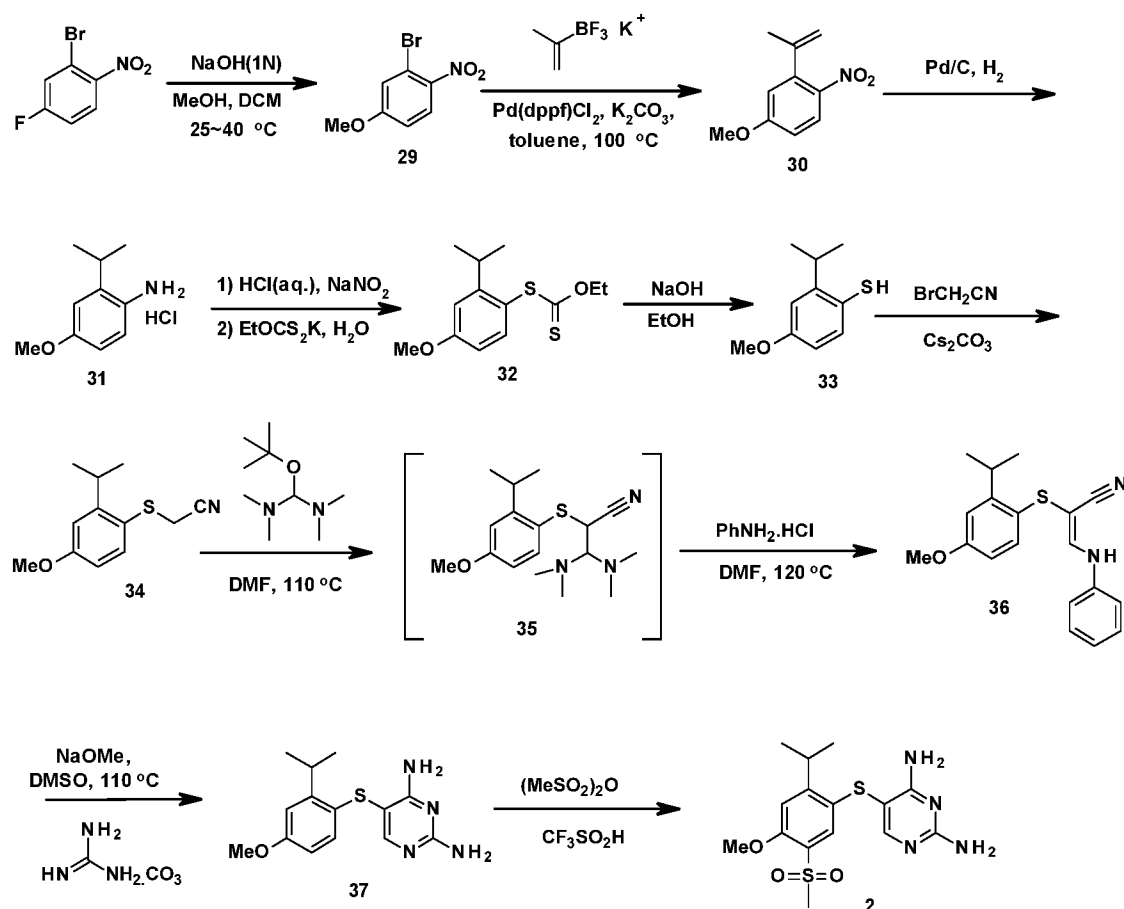
Scheme F
