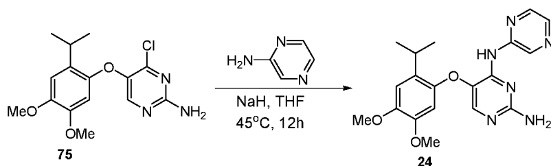
Scheme 30
