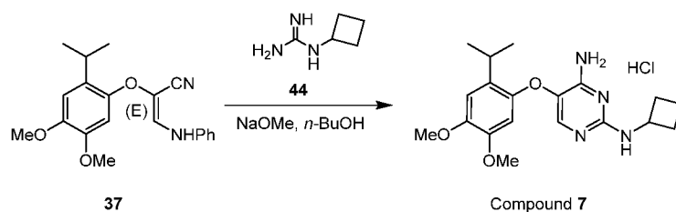
Scheme 10
