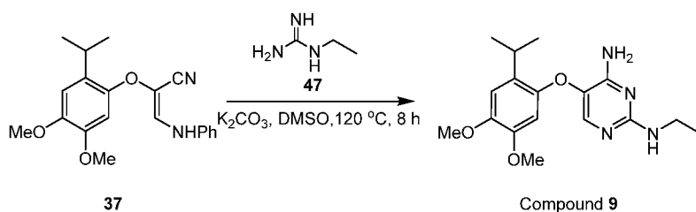
Scheme 13
