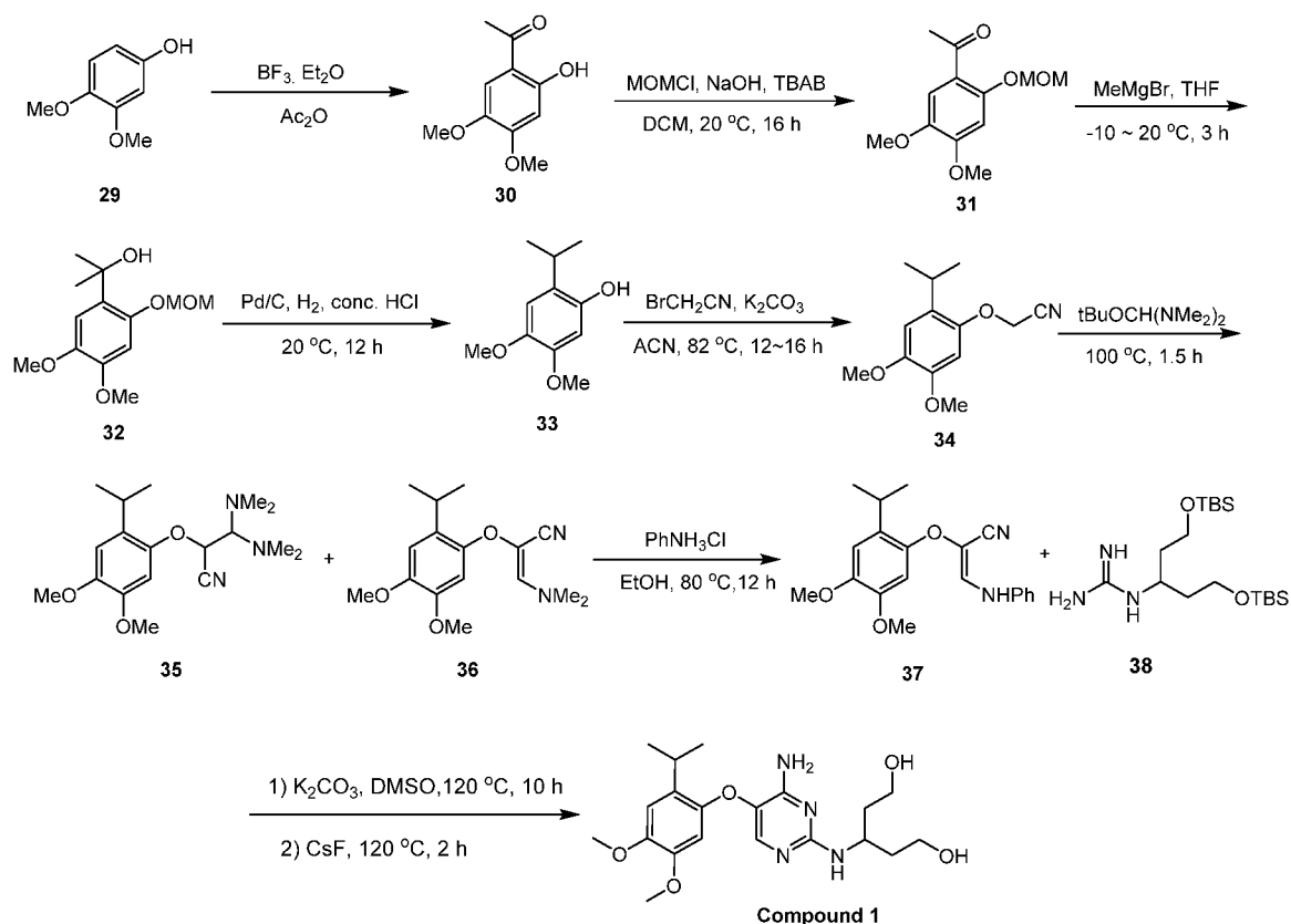
Scheme 4
