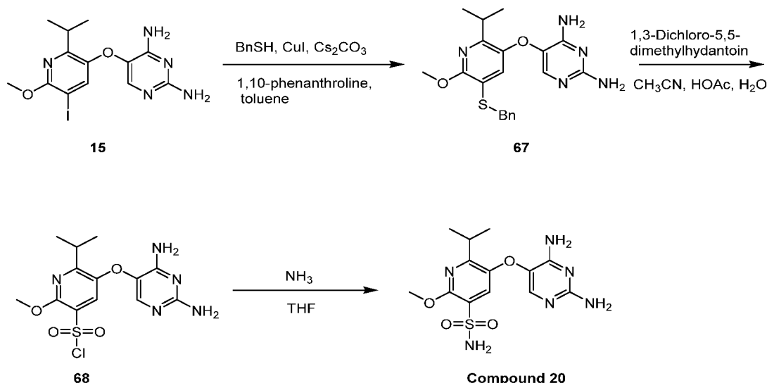
Scheme Z
