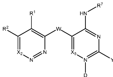
Formula 1h.
