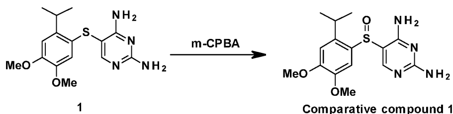
Scheme Q
