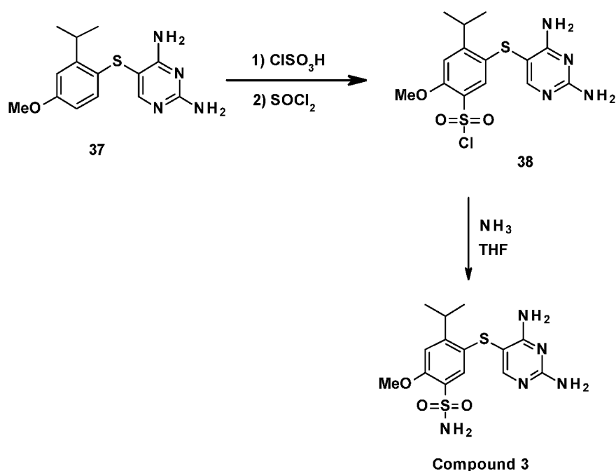
Scheme G
