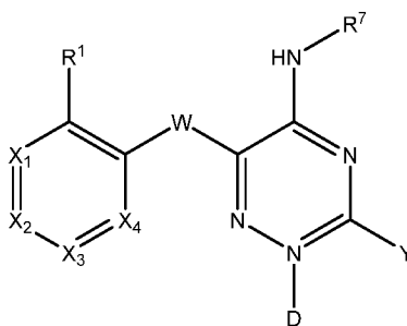
Formula 1l.
