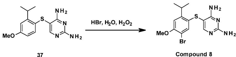
Scheme L
