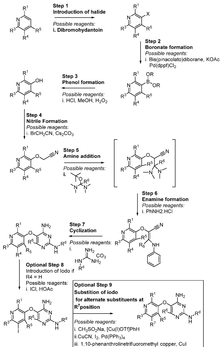
Scheme C
