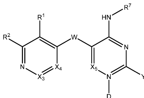
Formula 1c.
