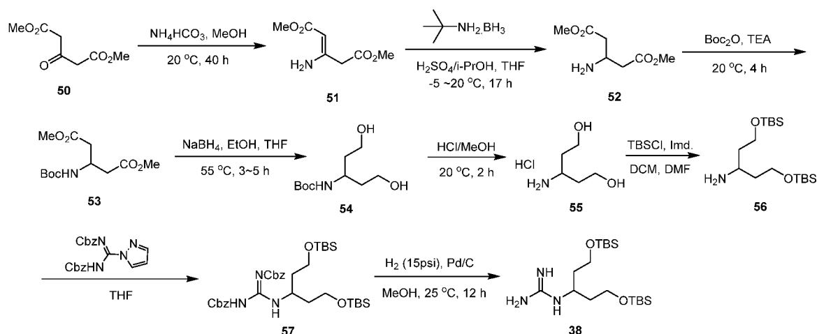
Scheme 16
