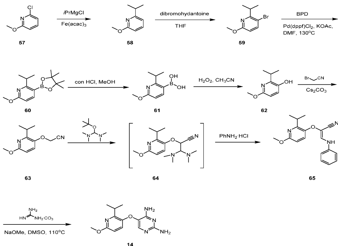
Scheme T
