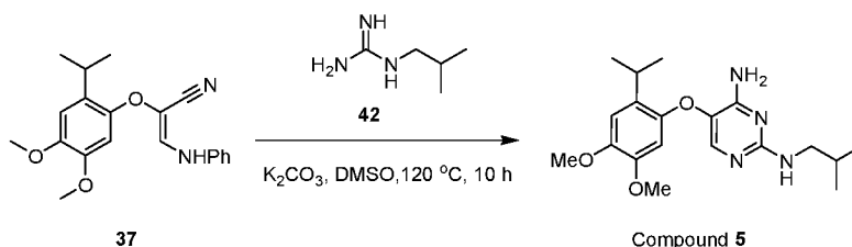
Scheme 8
