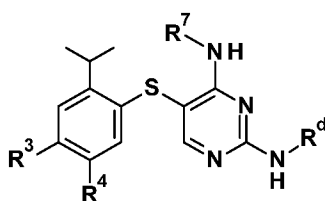
Formula 3
