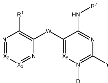
Formula 1k.
