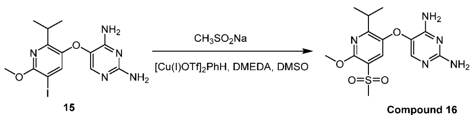
Scheme V
