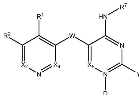
Formula 1d.
