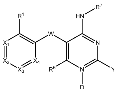
Formula 1m,
