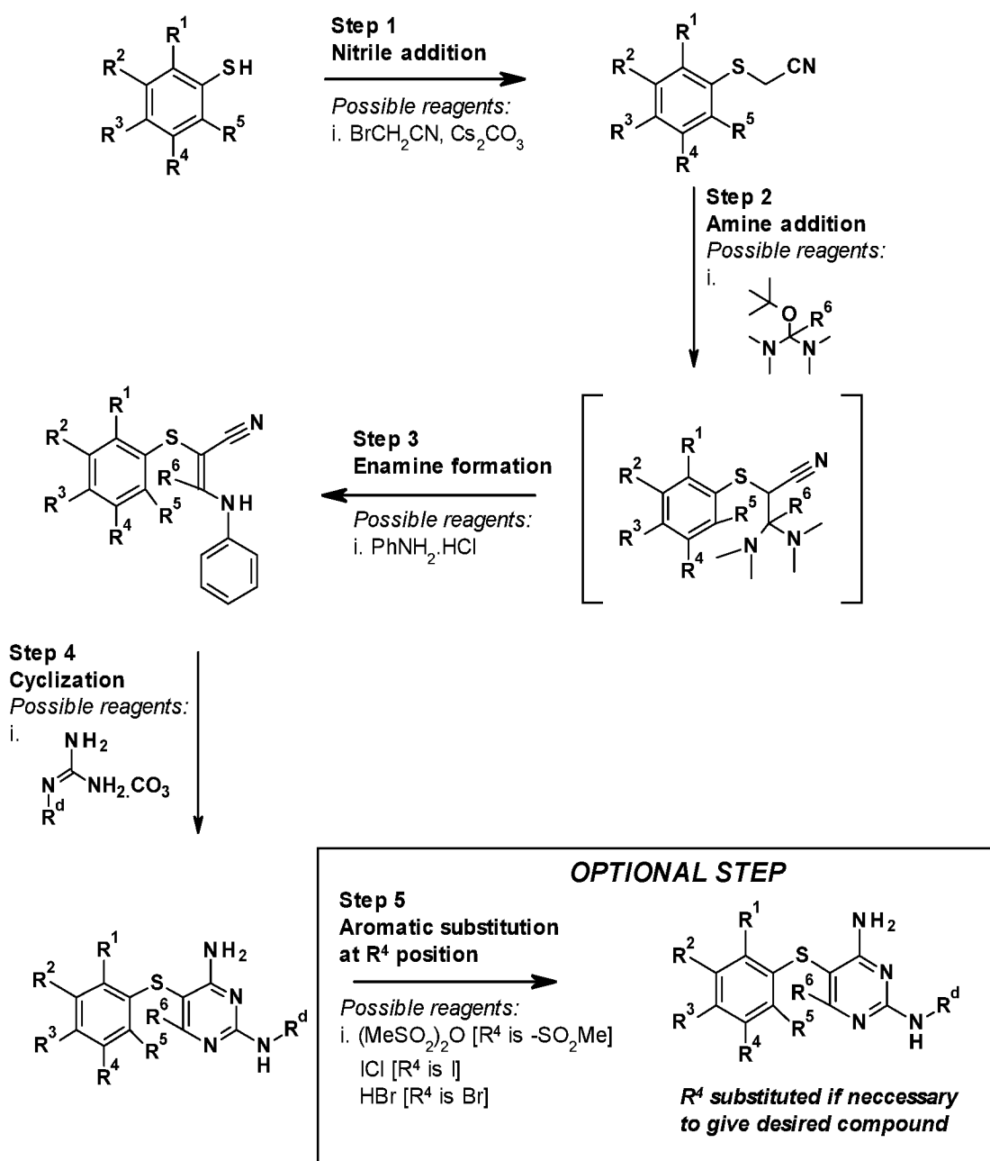
Scheme B
