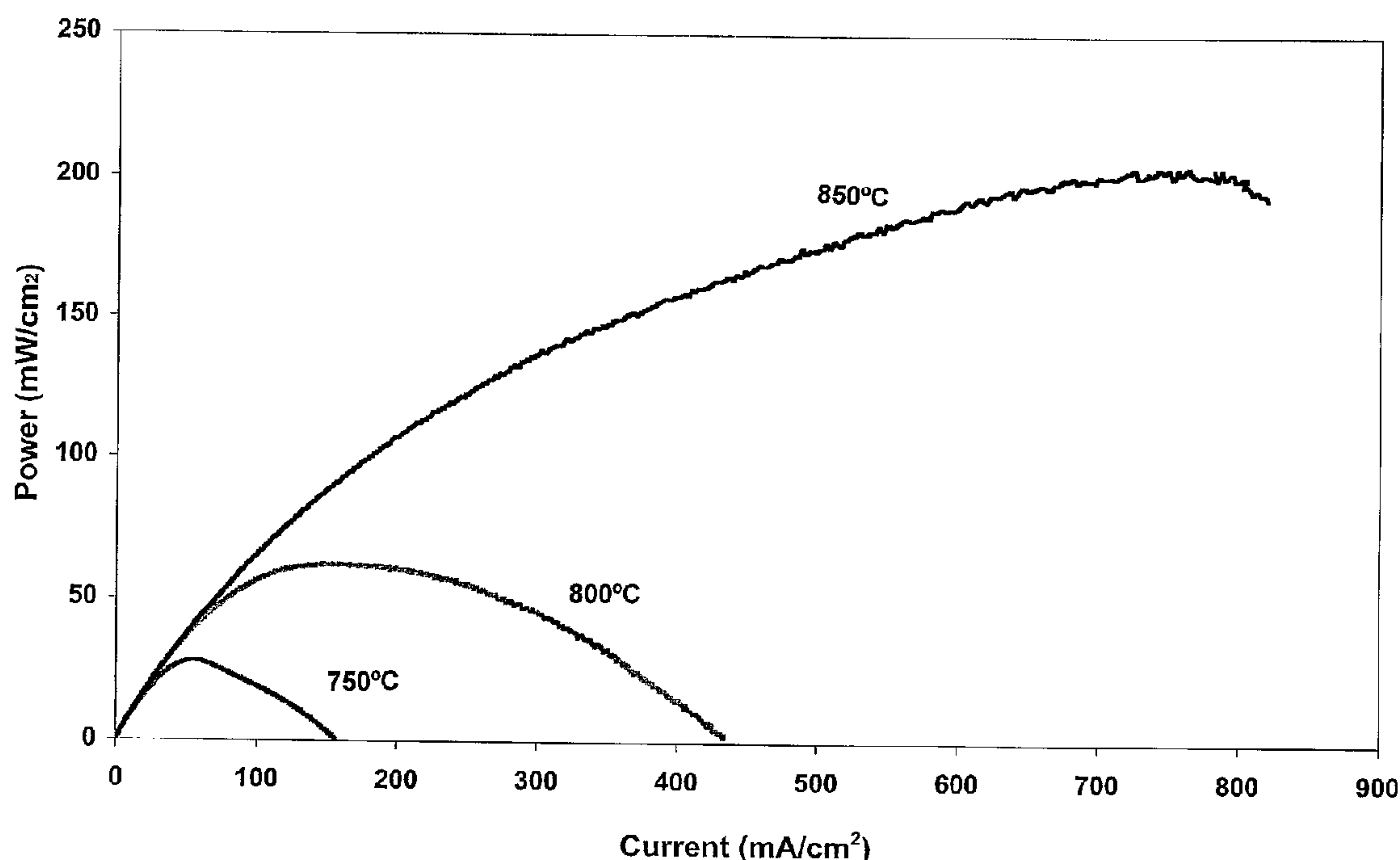
I-P curves for (MoS 2 +NiS+Ag+YSZ) anode
