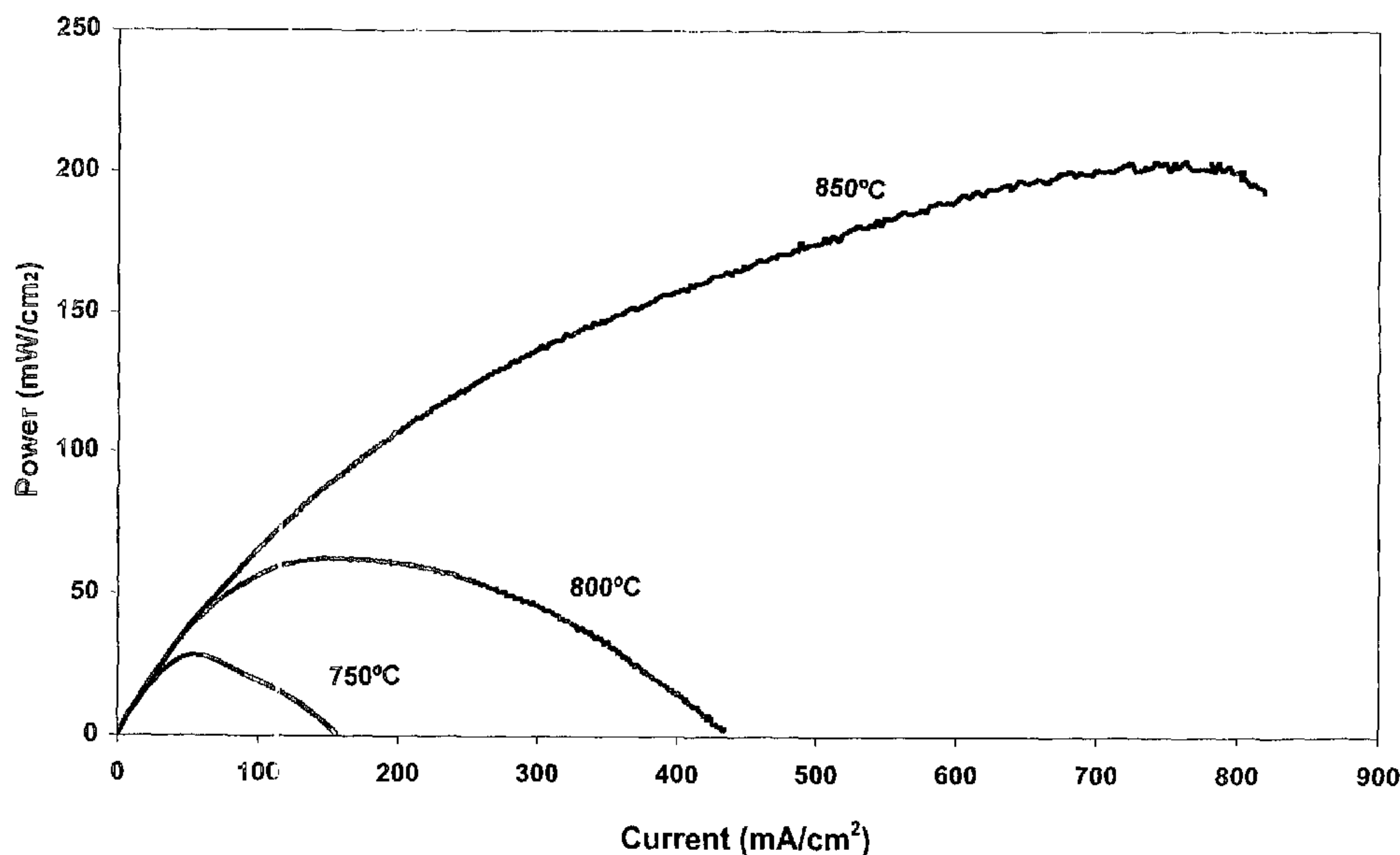
I-P curves for (MoS 2 +NiS+Ag+YSZ) anode
