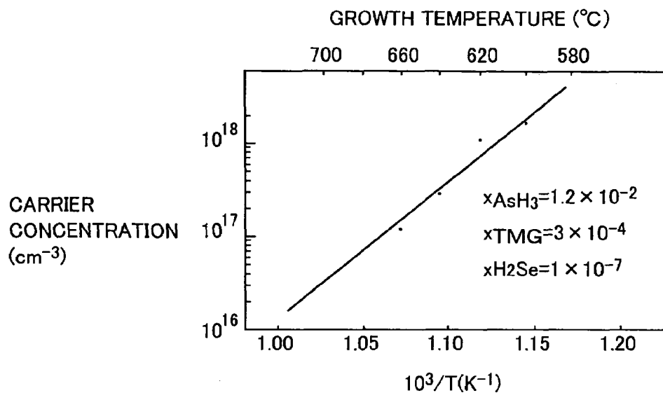
RELATION BETWEEN \text{H}_2\text{Se} DOPE CARRIER CONCENTRATIONS AND CRYSTAL GROWTH TEMPERATURES
