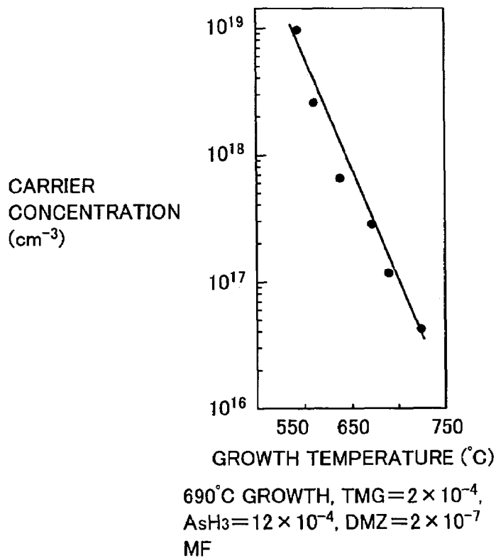
RELATION BETWEEN Zn DOPE CARRIER CONCENTRATIONS AND CRYSTAL GROWTH TEMPERATURES
