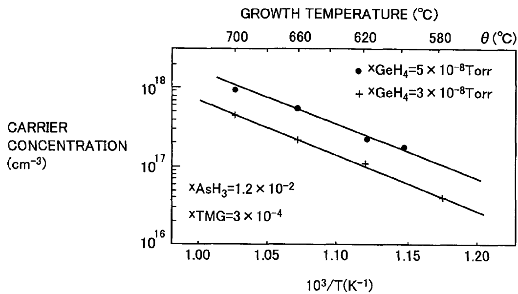
RELATION BETWEEN \text{GeH}_4 DOPE CARRIER CONCENTRATIONS AND CRYSTAL GROWTH TEMPERATURES
