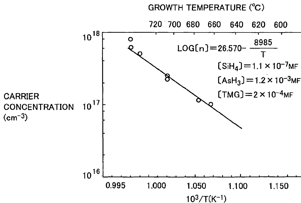
RELATION BETWEEN \text{SiH}_4 DOPE CARRIER CONCENTRATIONS AND CRYSTAL GROWTH TEMPERATURES
