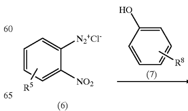
Reaction scheme-3
