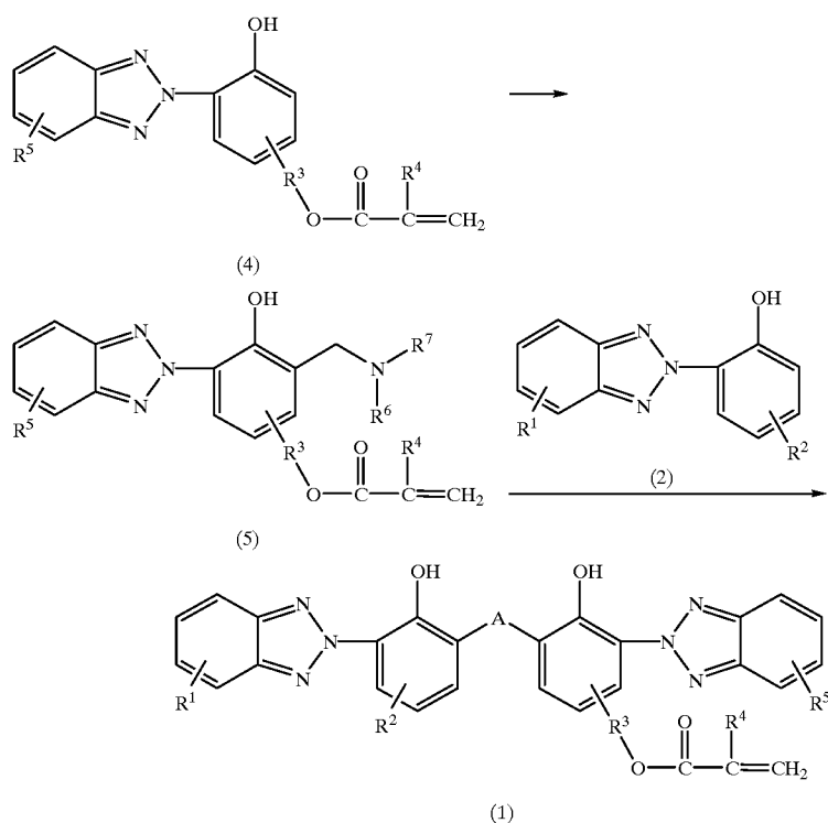
Reaction scheme-2
