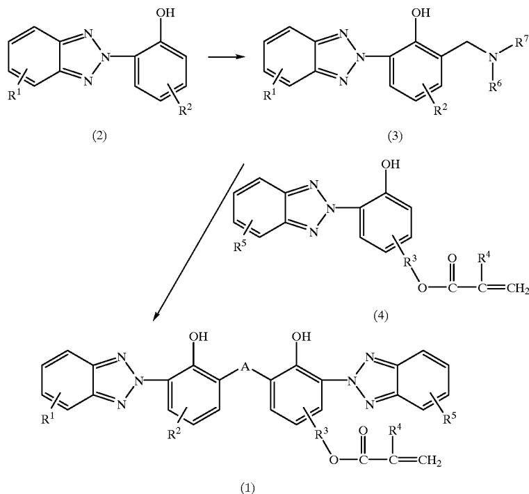
Reaction scheme-1
