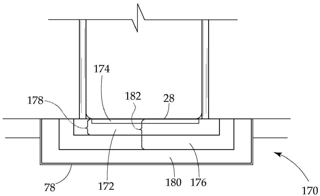
Front View Plate 1, 2 and 3 Closed
