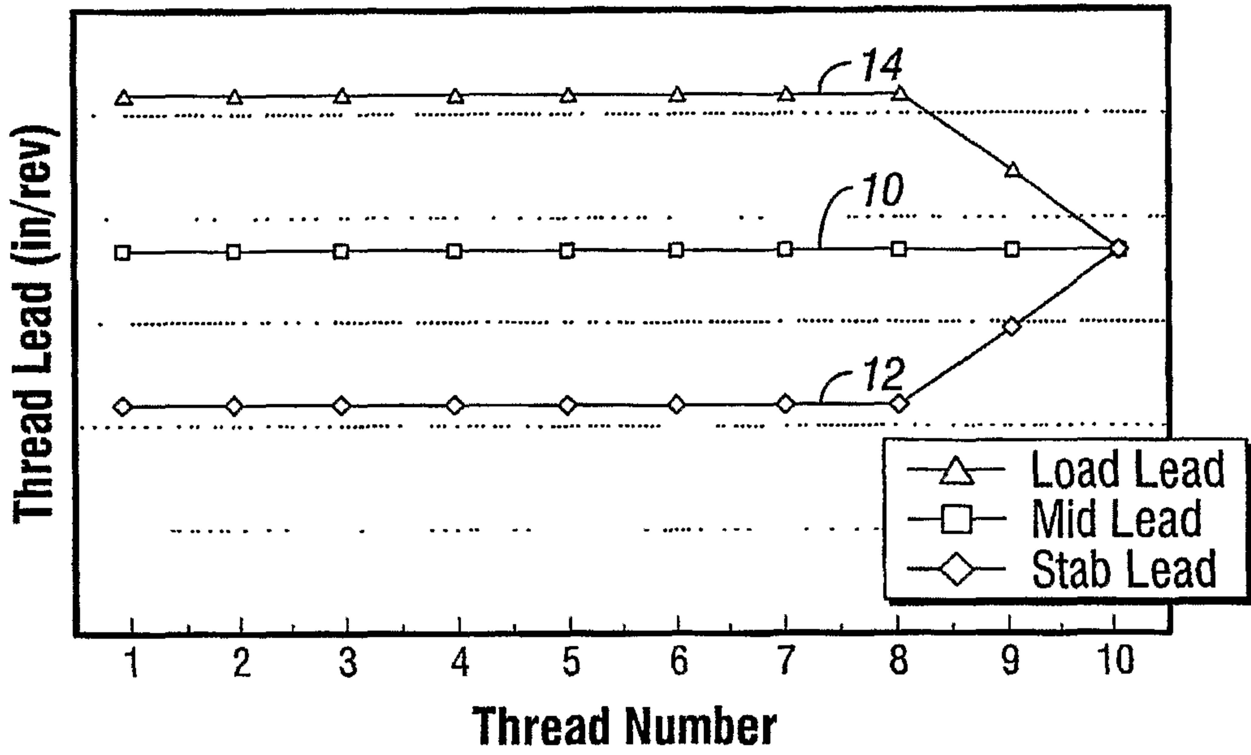
FIG. 3C (Prior Art)
