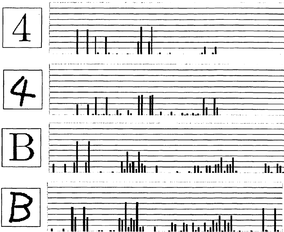
EXAMPLES OF ONE-DIMENSIONAL NUMERIC VALUES (VECTORS) GENERATED BY DISTRIBUTION MAPS (NUMERIC CHARACTER "4" OF 72 PT EUCLID FONT AND HAND WRITTEN CHARACTER "4")
