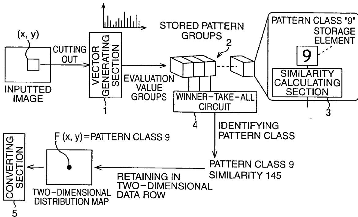
SCHEMATIC DIAGRAM OF WHOLE SYSTEM
