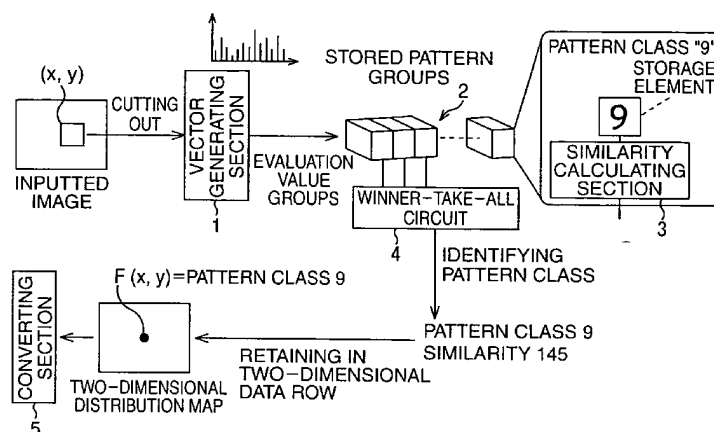
SCHEMATIC DIAGRAM OF WHOLE SYSTEM
