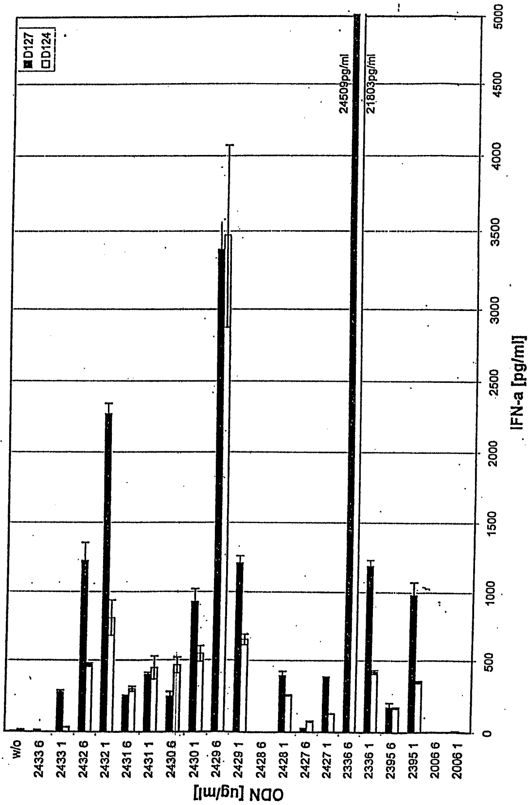
FIGURE 8, IFN-a secretion 2395 and variants (451)
