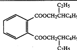
Solv-7: Bis(2-ethylhexyl) phthalate
