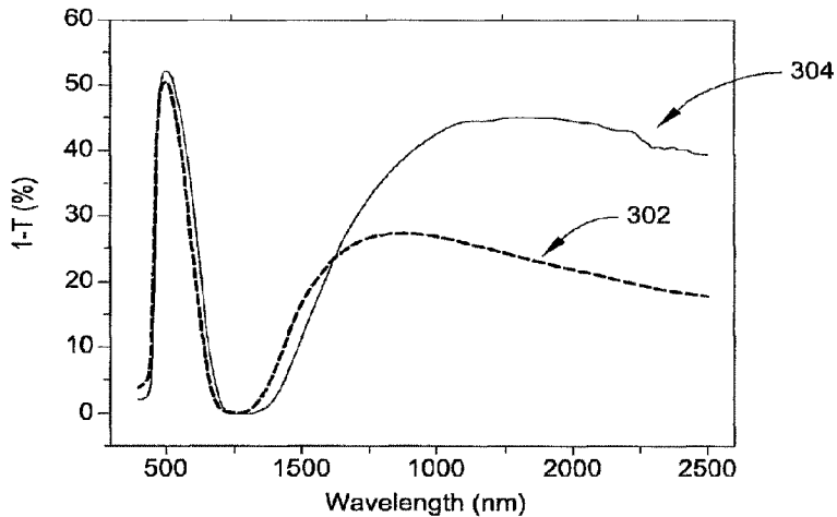
Polyaniline Film Absorption
