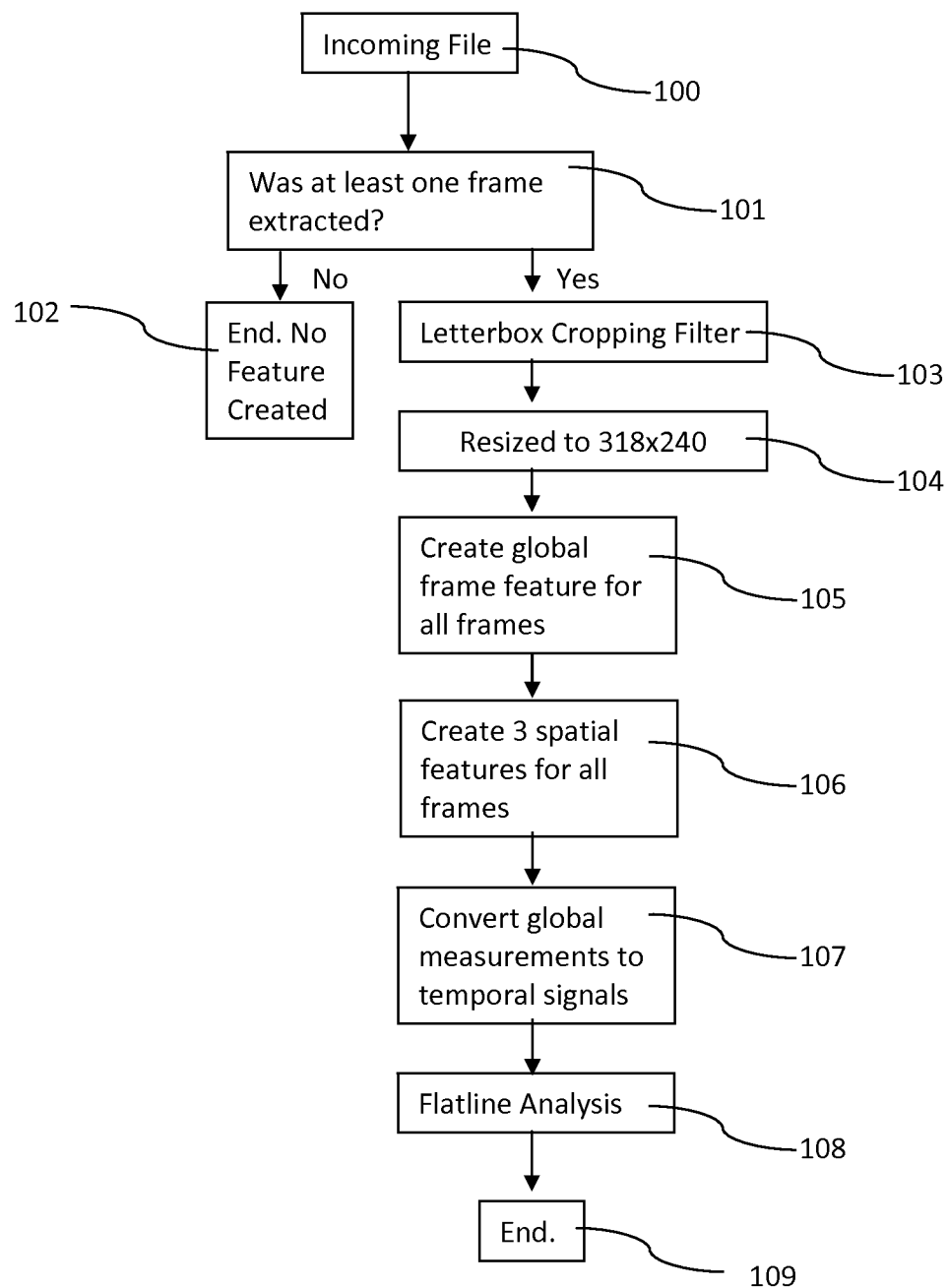
Video Feature Extraction Process Flow Chart
