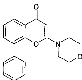
LY 294002
