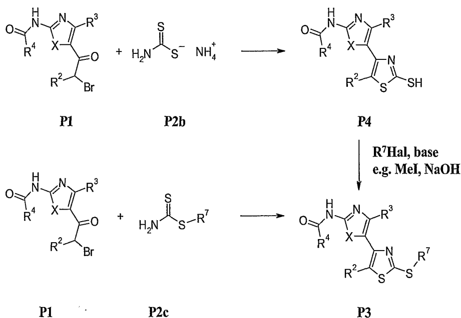
Scheme 7
