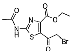
Intermediate 6
