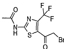
Intermediate 5
