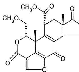
Wortmannin
