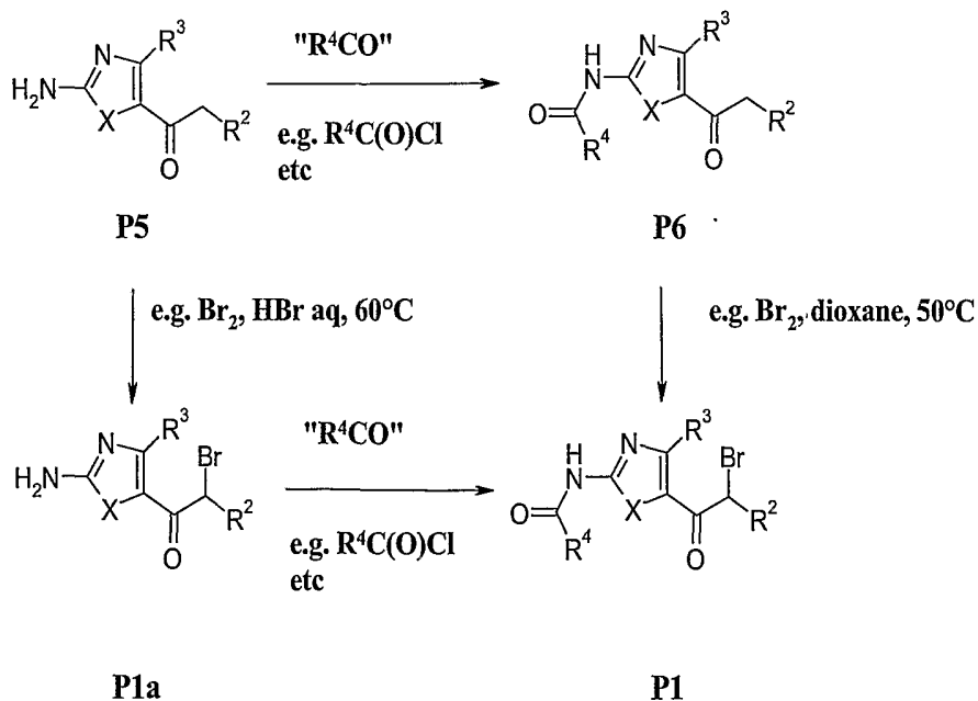
Scheme 9
