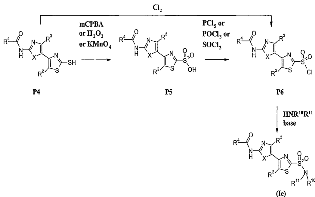
Scheme 6
