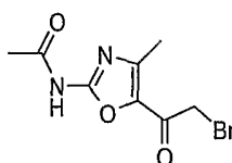
Intermediate 3
