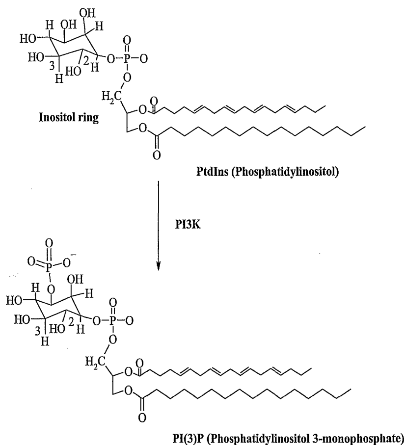
Scheme A
