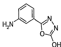
Amine 1
