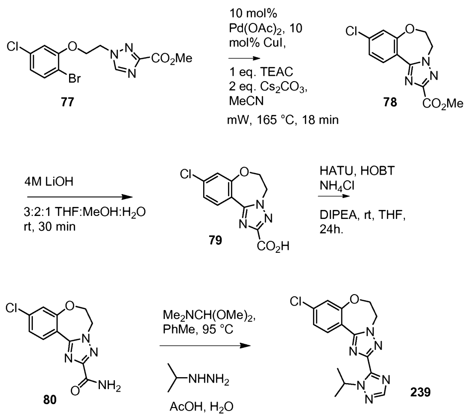
SCHEME 17
