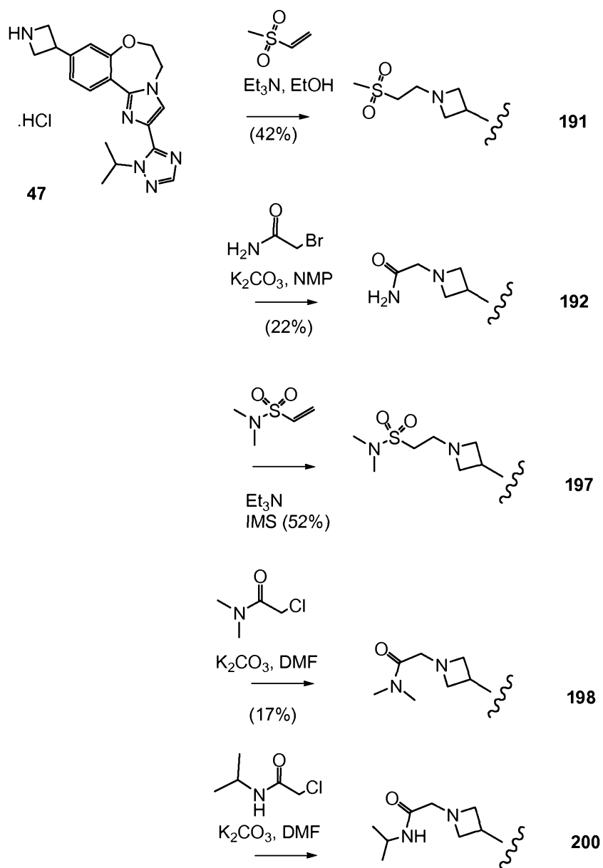
SCHEME 10
