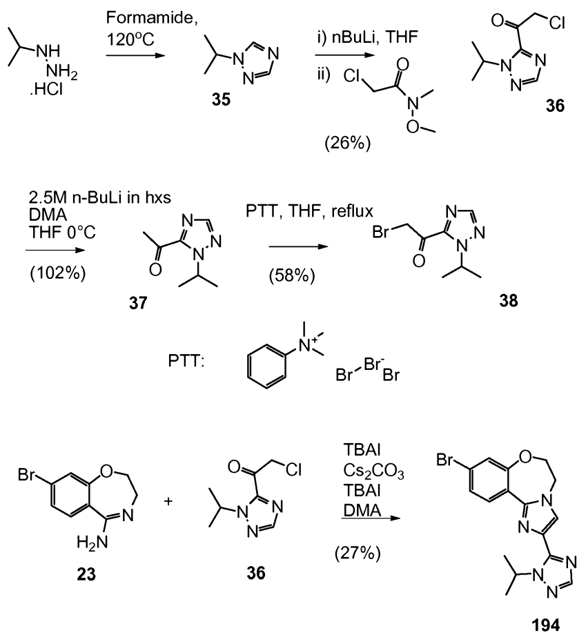
SCHEME 7
