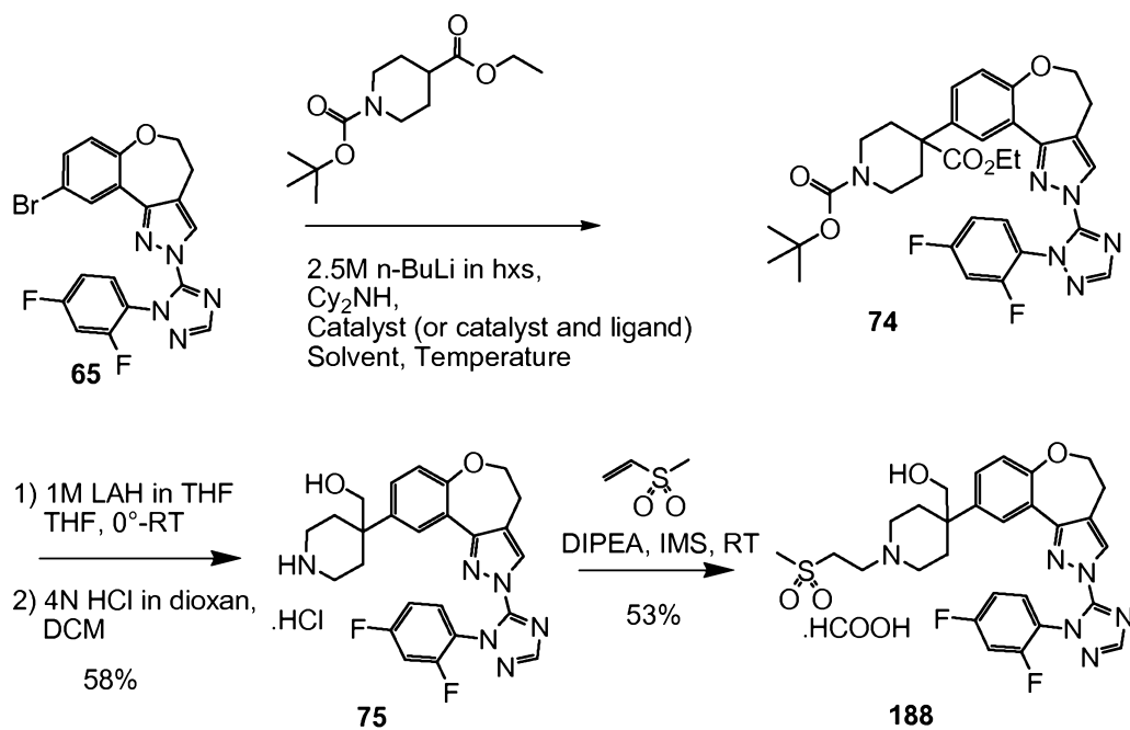
SCHEME 16
