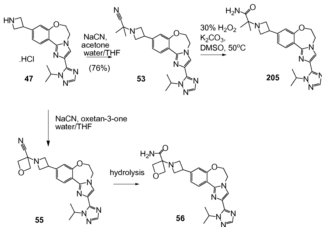
SCHEME 11
