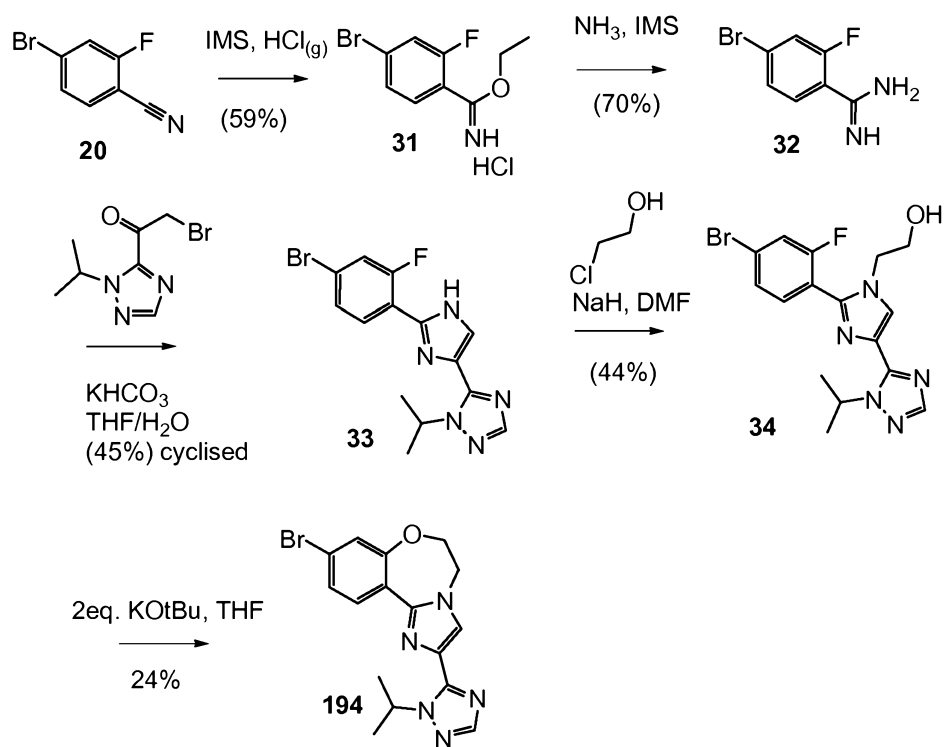
SCHEME 6
