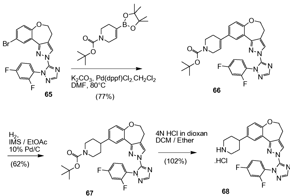
SCHEME 14
