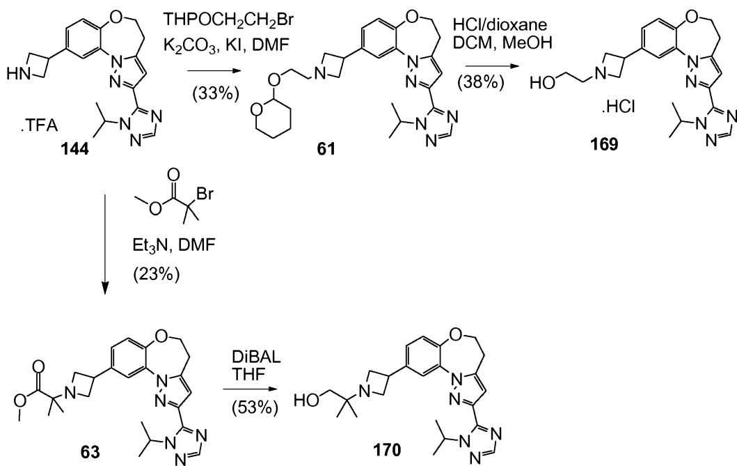
SCHEME 13
