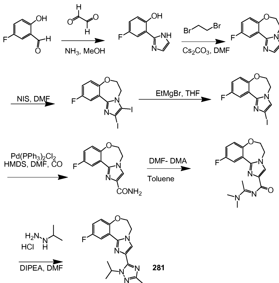
SCHEME 20
