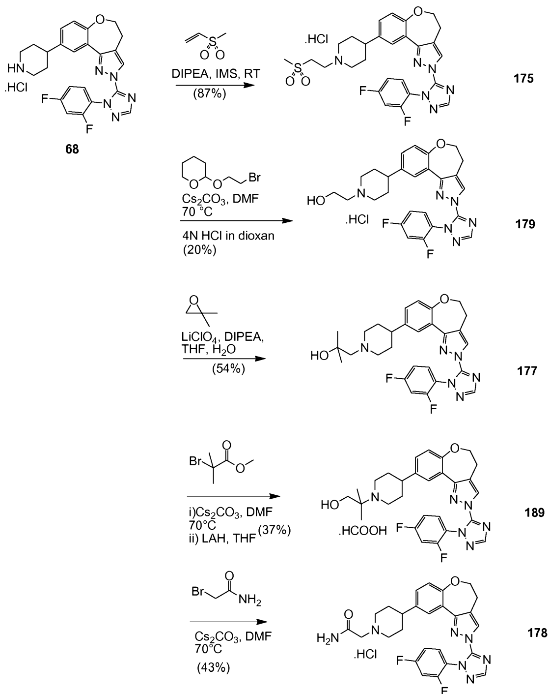
SCHEME 15
