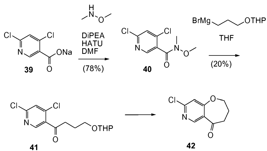
SCHEME 8
