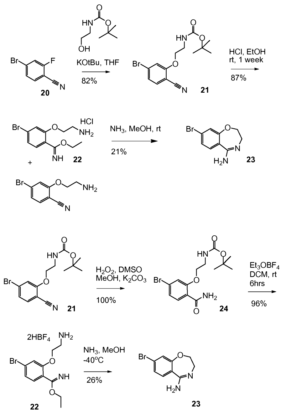
SCHEME 4
