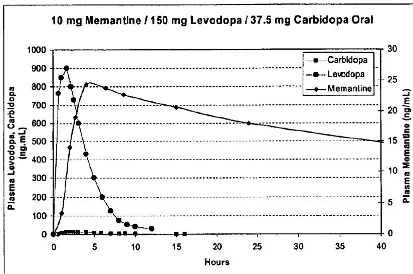
Figure 7: Target Pharmacokinetics
