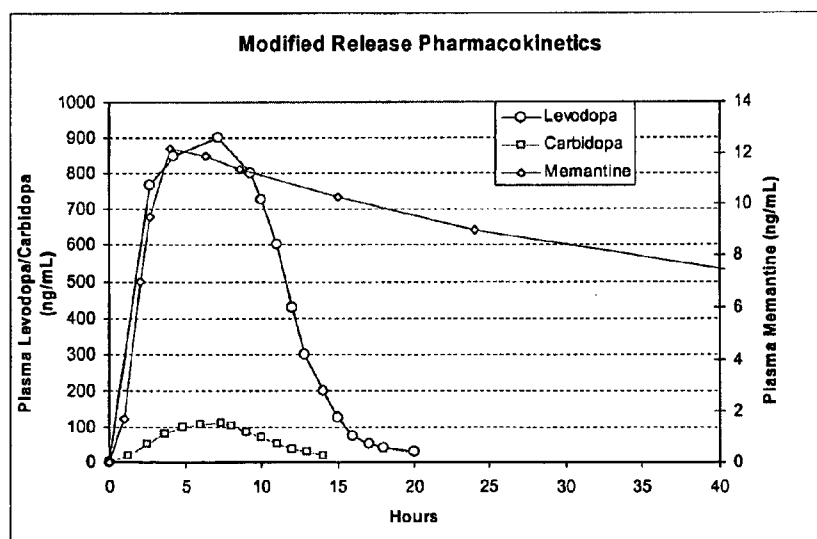
Figure 7: Target Pharmacokinetics
