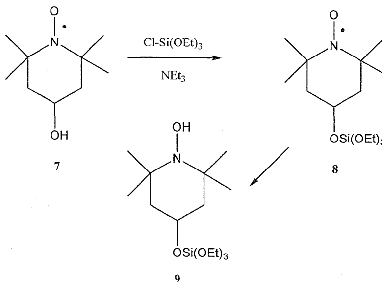
Scheme 6. Synthesis of a nitroxyl radical-containing organosilane monomer.
