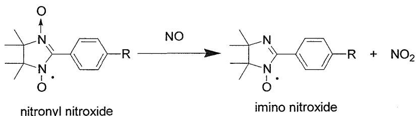
Scheme 2. Oxidation of NO using a nitronyl nitroxide active site.
