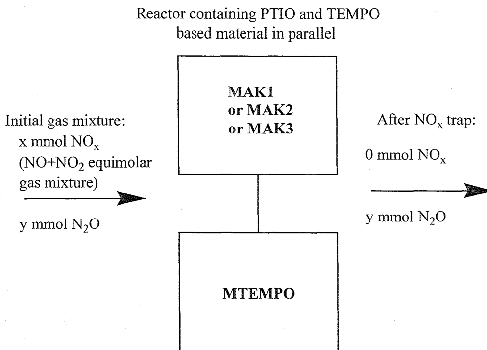
Scheme 12. Reaction of mixture of nitronyl nitroxide-based (MAK1, MAK2, MAK3) and nitroxyl radical-based (MTEMPO) materials functioning in a parallel configuration for the complete removal of NO x .
