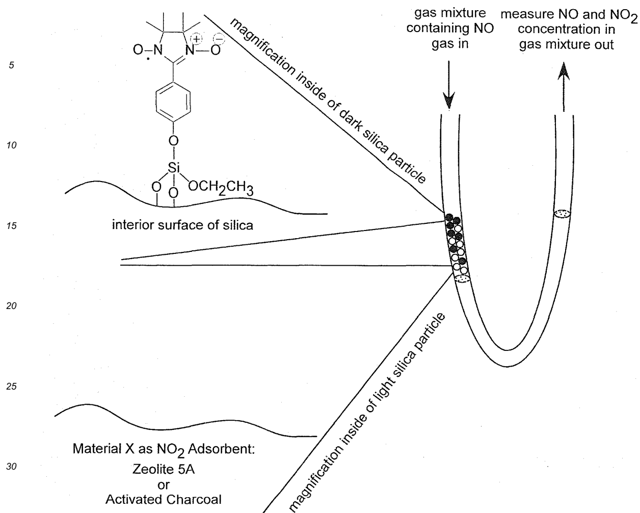
Scheme 16. U-tube reactor configuration used to evaluate mixtures of MNN1 and material X for NO removal from a gas mixture.
