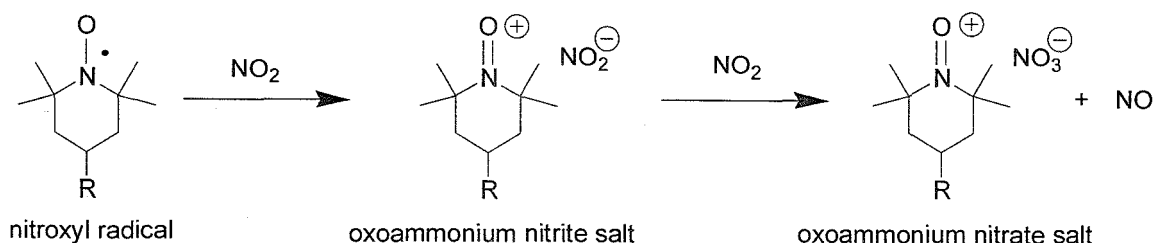
Scheme 1. Sequential reaction of nitroxyl radical site with NO 2 .
