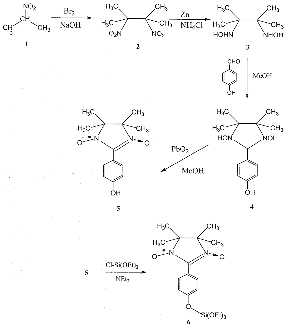
Scheme 5. Steps for synthesizing a nitronyl nitroxide-containing organosilane monomer.
