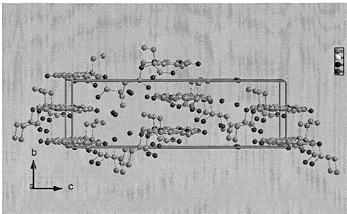
Fig. 5. Three Dimentional Crystal Structure of C_{23}H_{20}N_2O_5 \cdot 3H_2O (b,c-dimentionations)
