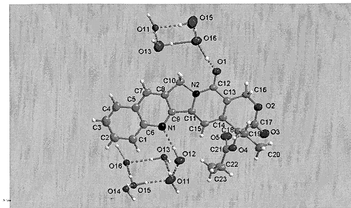
Fig. 1. Molecular Structure of C_{23}H_{20}N_2O_5 \cdot 3H_2O
