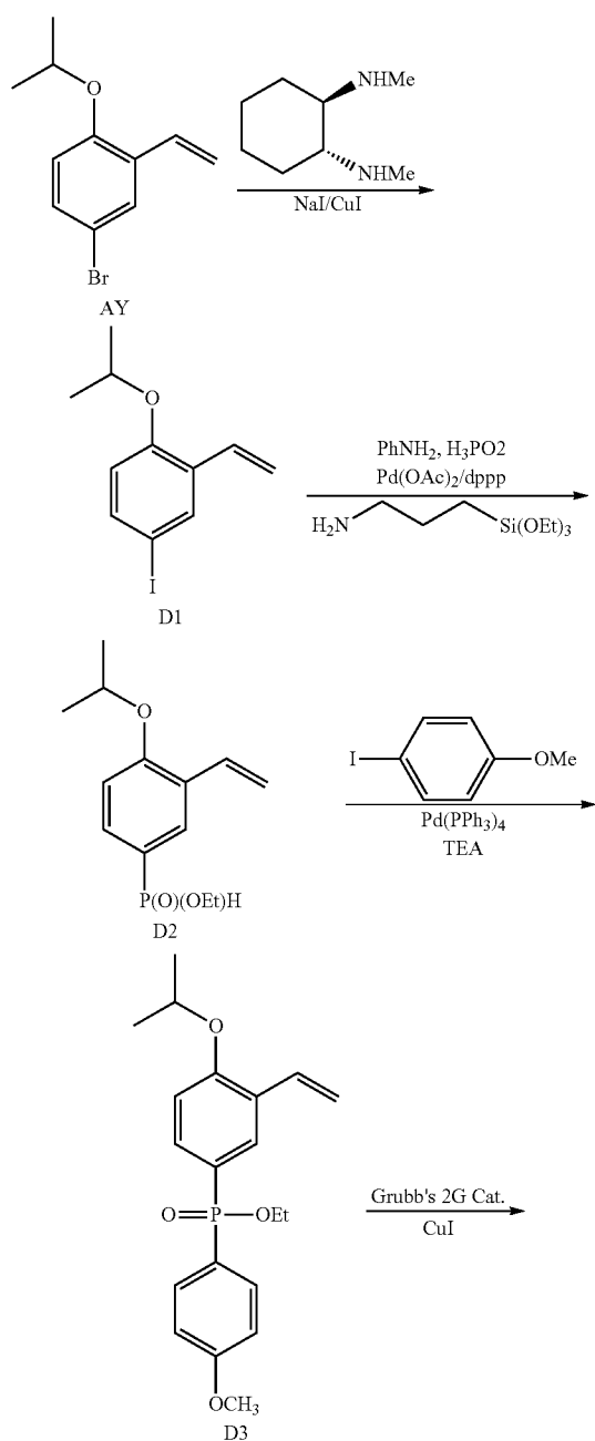
Scheme 4
