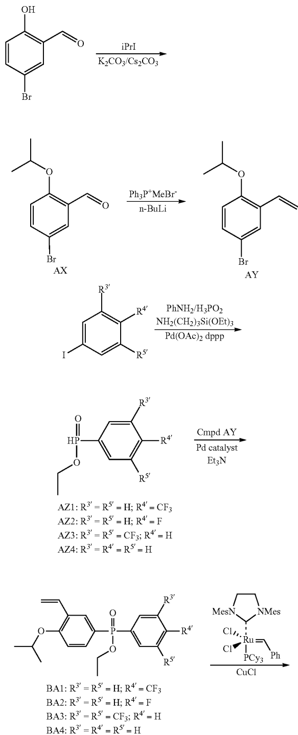
Scheme 2
