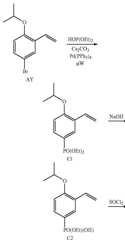
Scheme 3
