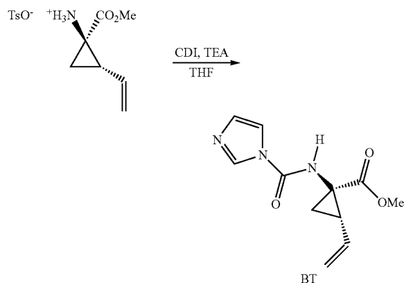
Scheme 12
