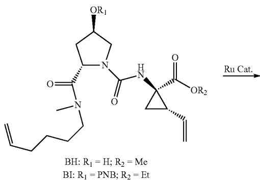
Scheme 8
