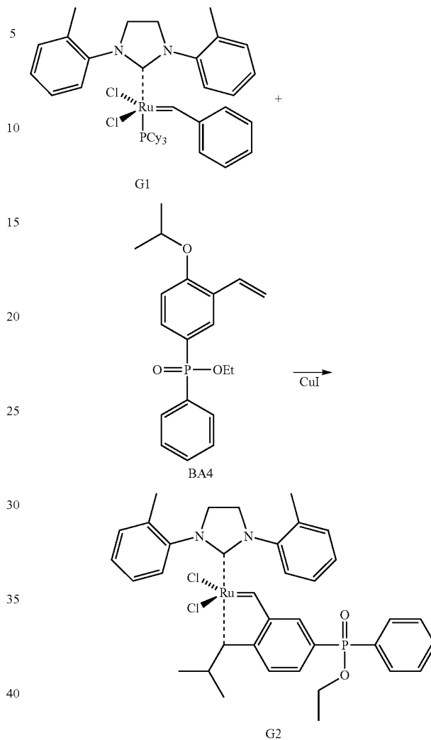
Scheme 6
