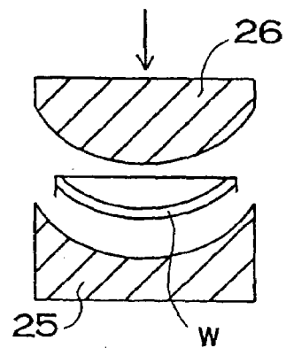
FIG. 3 (PRIOR ART)
