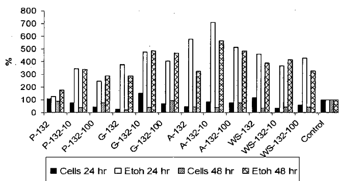
Chart 2C. % Growth and Ethanol Production for P. stipitis
