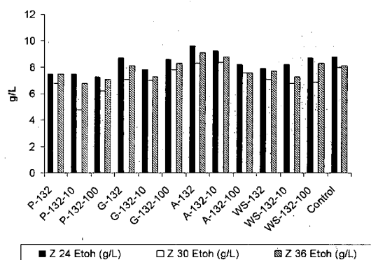
Chart 1B. Ethanol Concentrations for Z. mobilis
