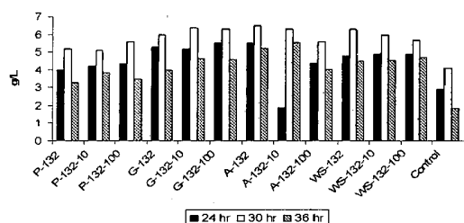
Chart 3B. Ethanol Concentrations for S. cerevisiae
