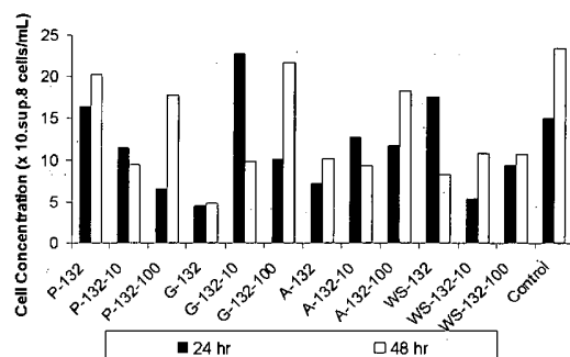
Chart 2A. Cell concentrations for P. stipitis
