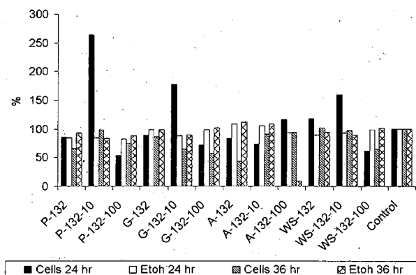
Chart 1C. % Growth and Ethanol Production for Z. mobilis
