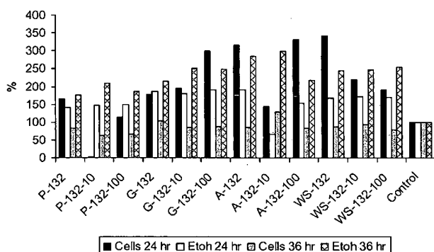
Chart 3C. % Growth and Ethanol Production for S. cerevisiae
