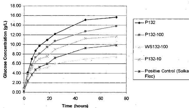
Chart 1. Glucose Concentration (Top 4 producers)
