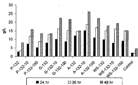
Chart 2B. Ethanol Concentrations for P. stipitis
