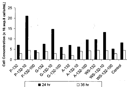
Chart 1A. Cell Concentrations for Z. mobilis
