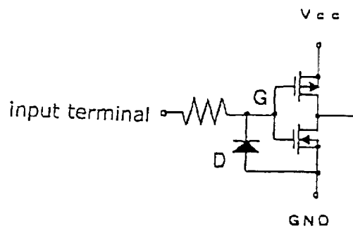
FIG. 8 (PRIOR ART)
