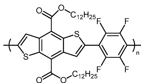
(polymer 1),
