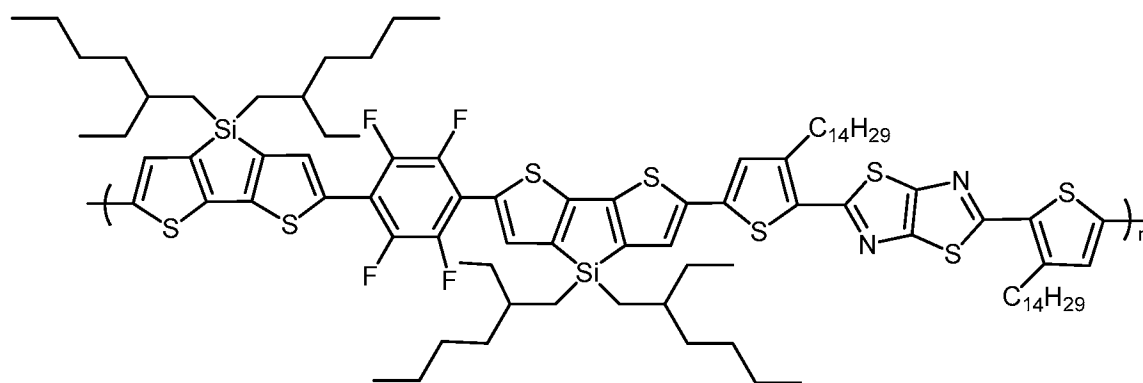
(polymer 3),
