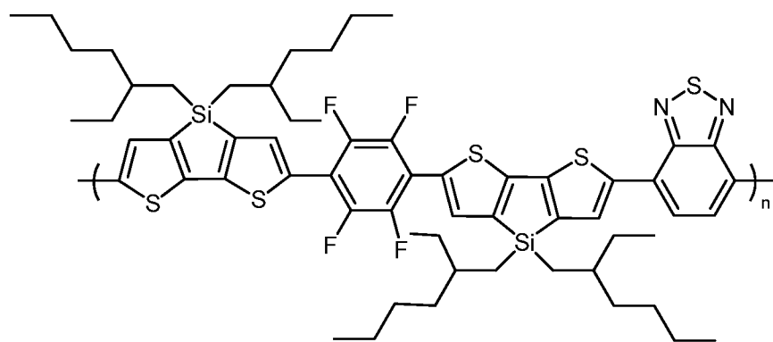
(polymer 1),
