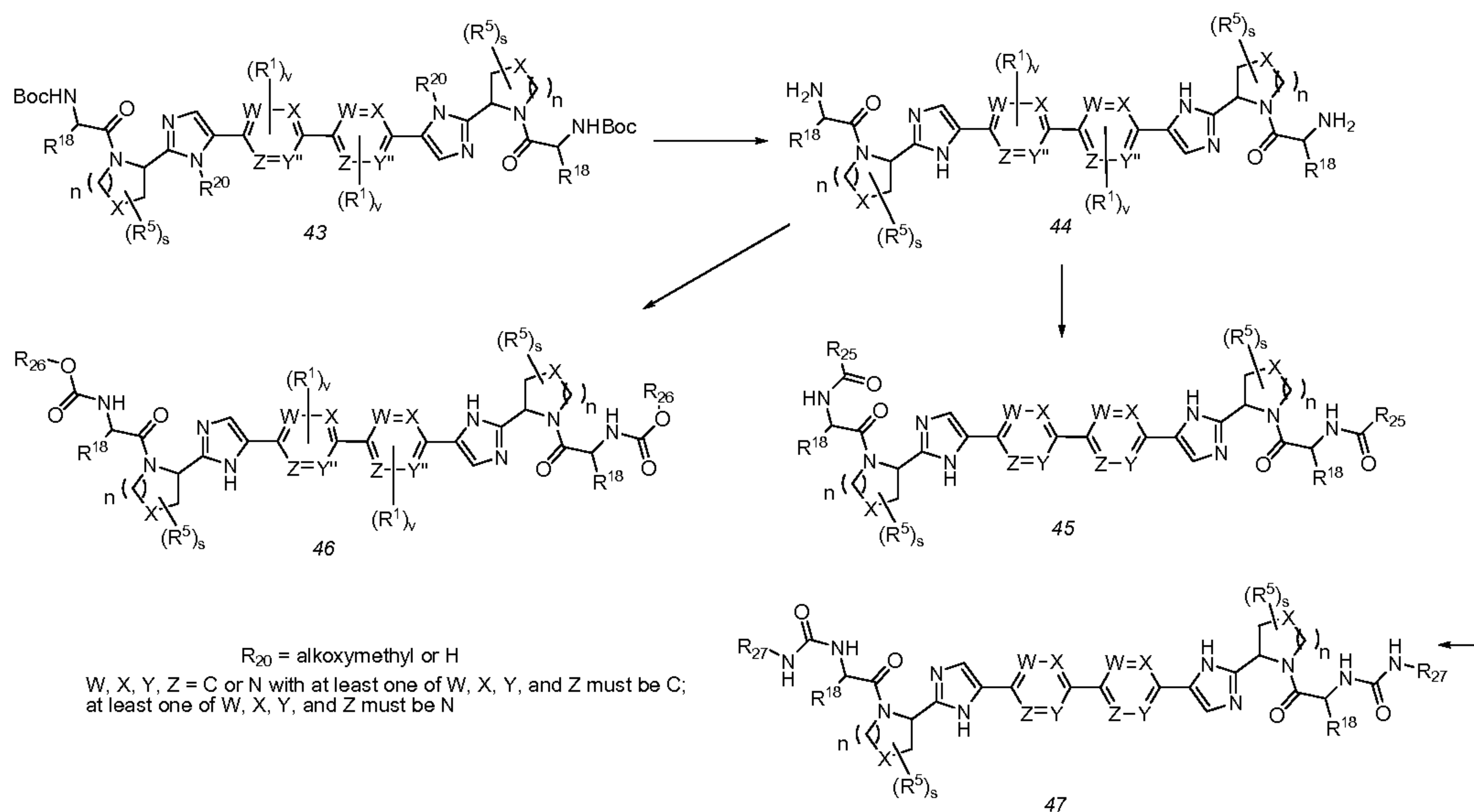
Scheme 10: Starting Material 29
