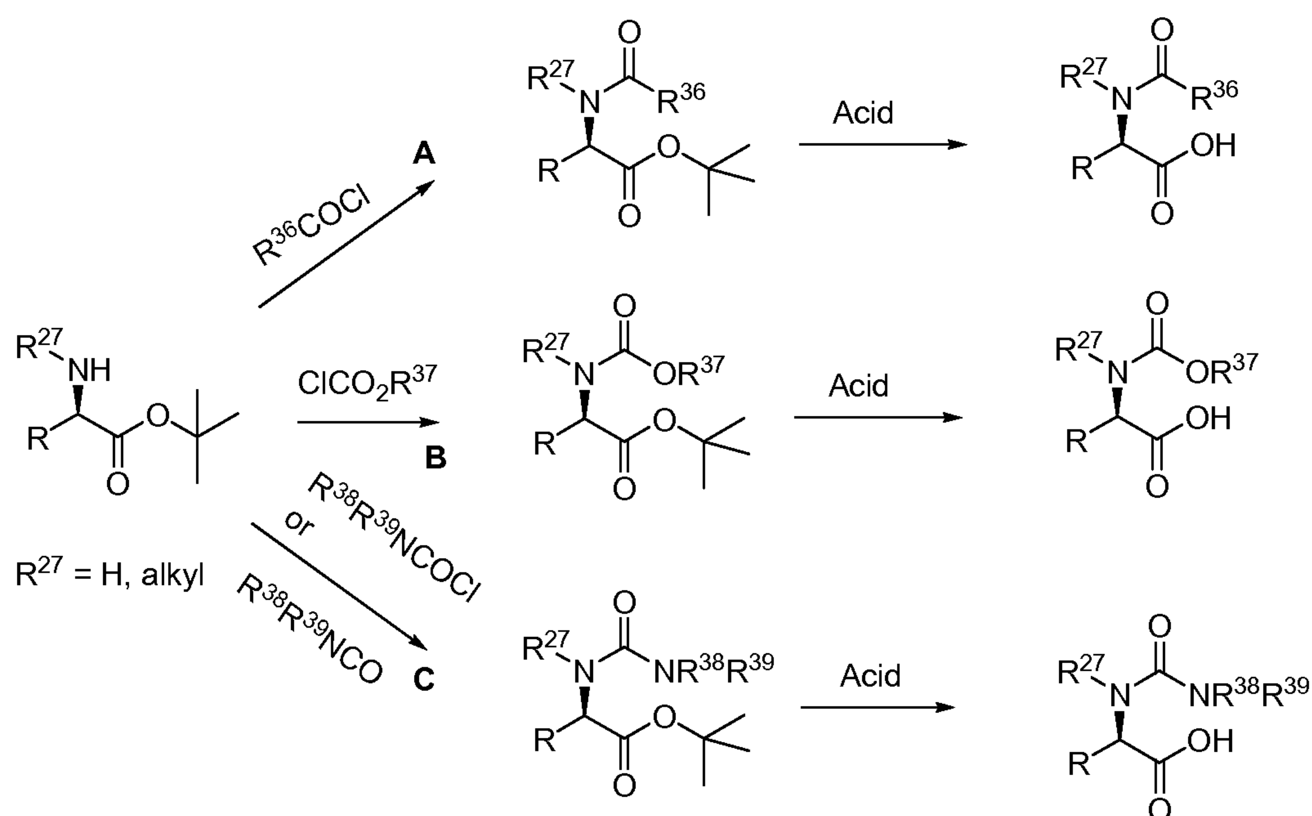
Scheme 13
