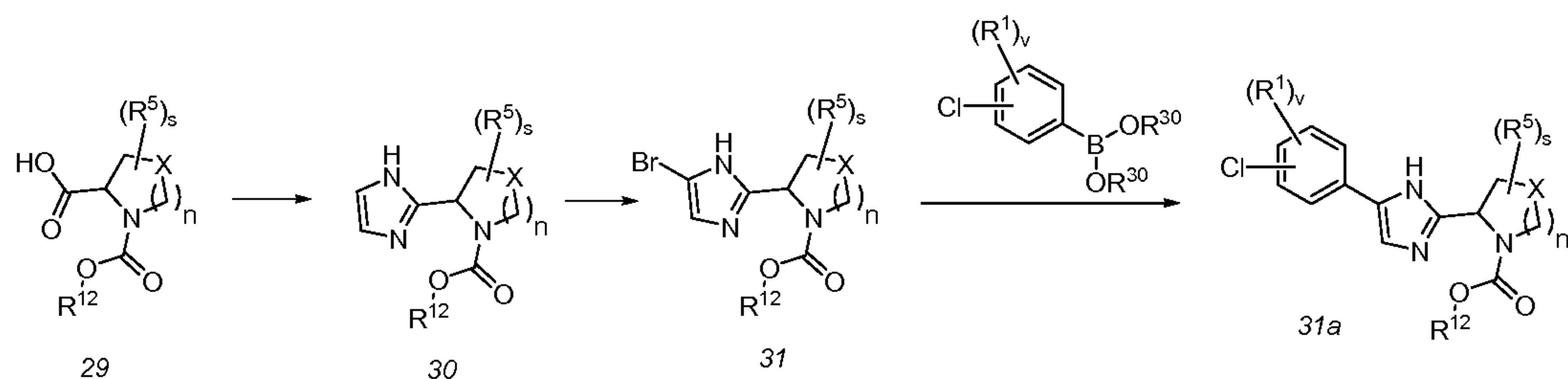
Scheme 7: Heteroaryls
