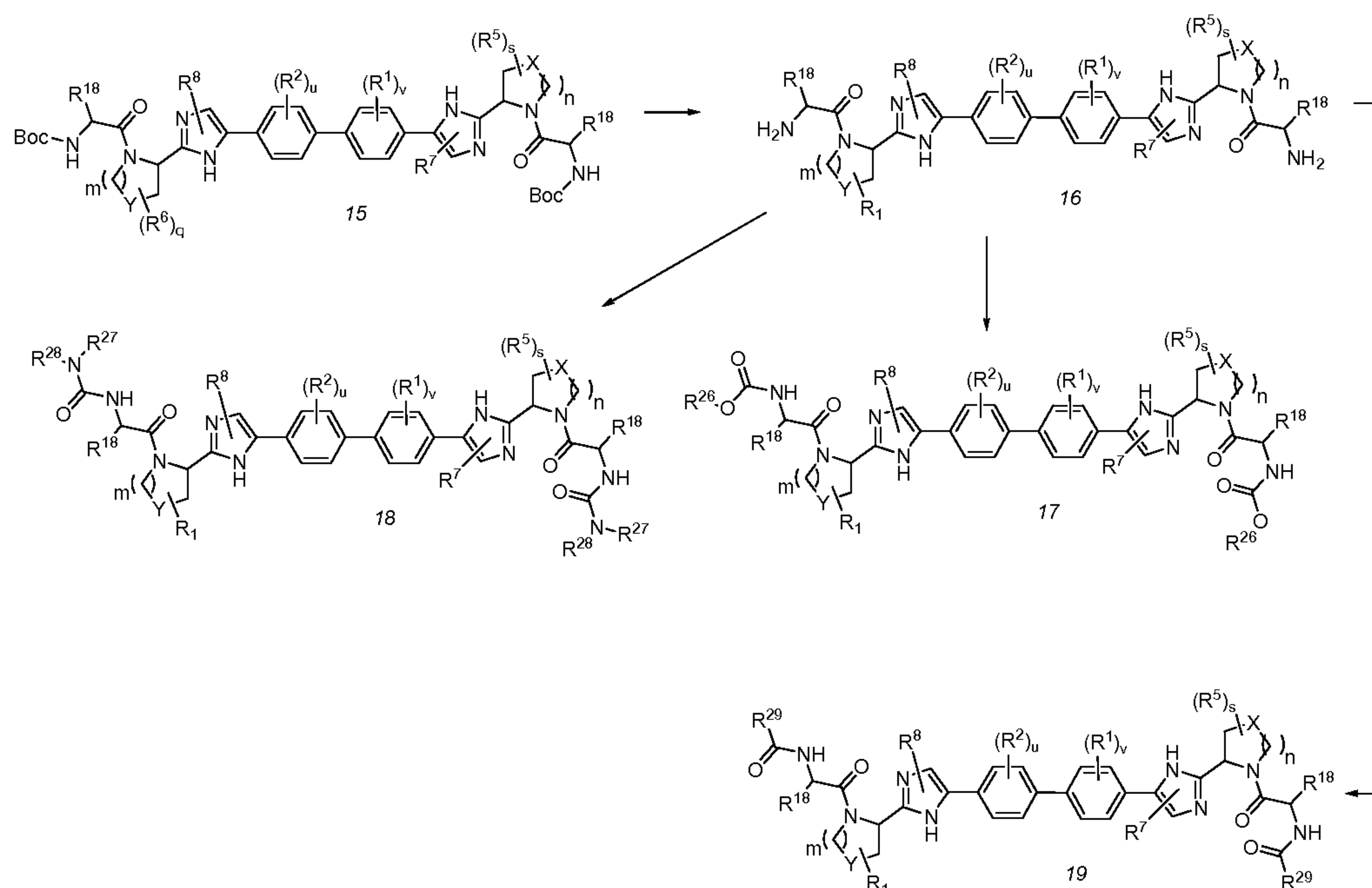
Scheme 4: Symmetric Biphenyls
