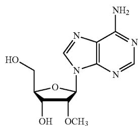
2'-O-methyl-adenosine
