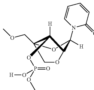
2',4'-BNA-2-pyridone
