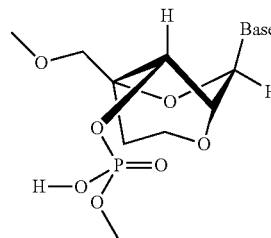
2',4'-ENA
