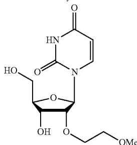
2'-O-methoxyethyl uridine
