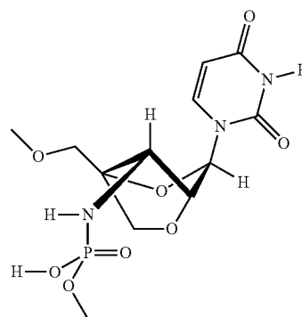
3'-amino-2',4'-BNA
