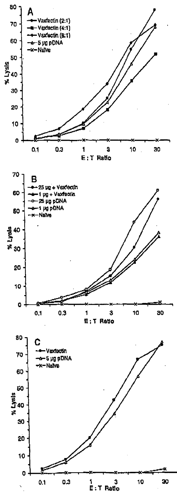
Vaccine, Hartikka et al., Figure 8
