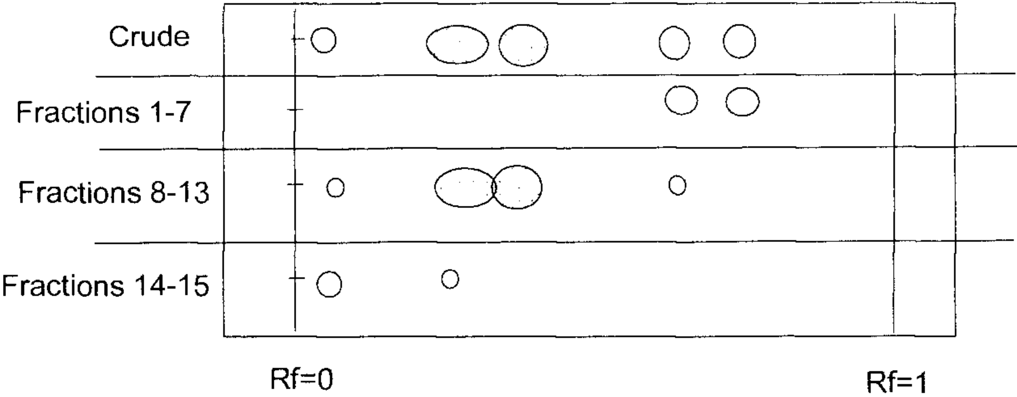
Schematic TLC profile of the collected fractions
