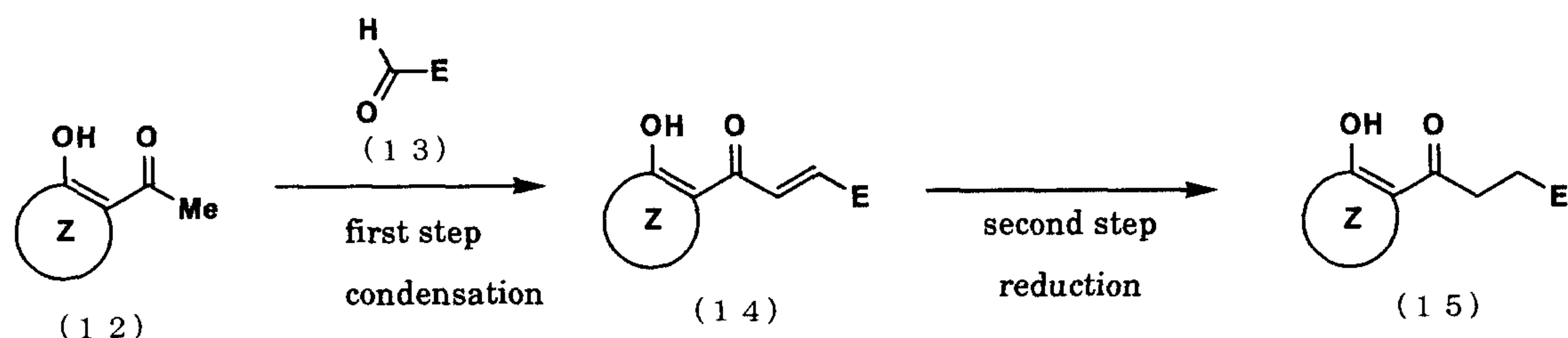
Reaction Scheme 4
