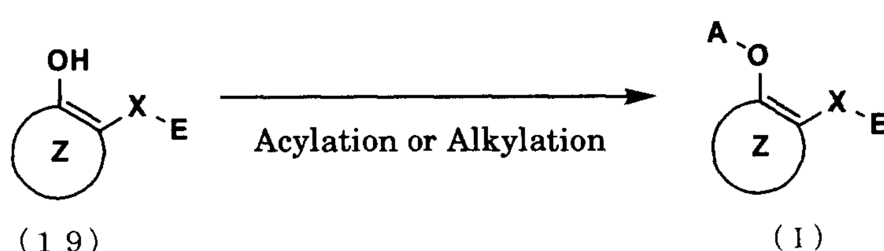
Reaction Scheme 6
