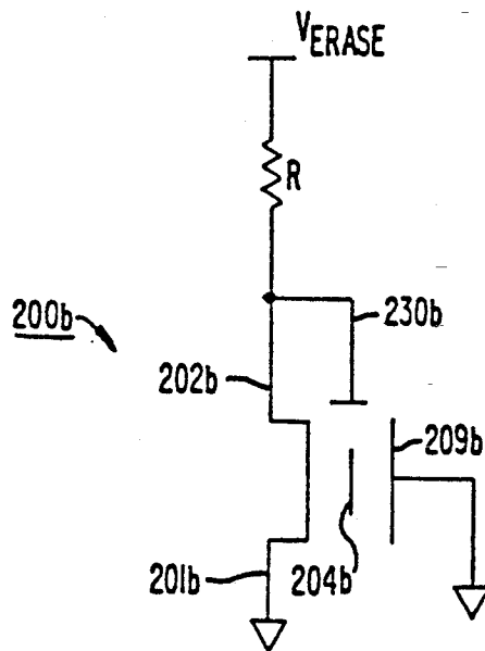
FIG. 2c. PRIOR ART
