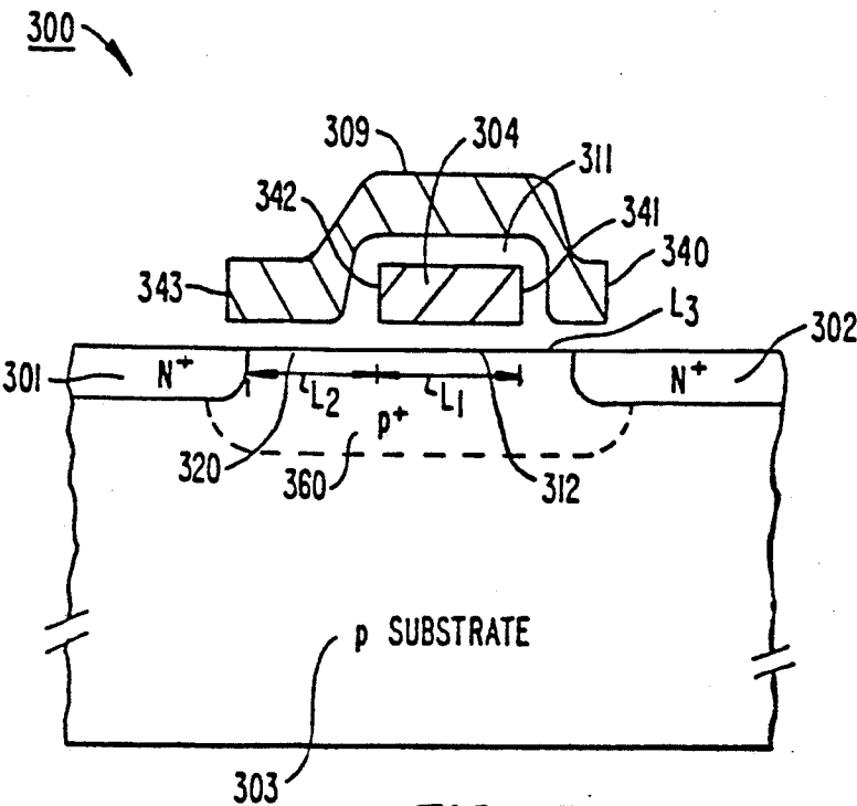
FIG. 3c. PRIOR ART
