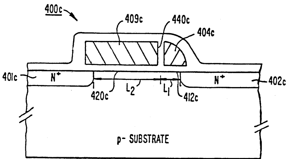
FIG. 4c. PRIOR ART
