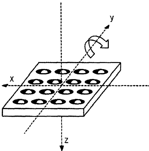
FIG. 23C RELATED ART
