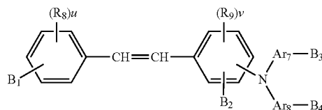
Chemical formula 20
