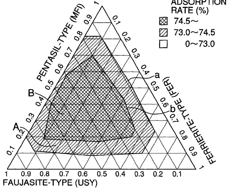
FIG. 7 RATIO OF ZEOLITES AND ADSORPTION RATE
