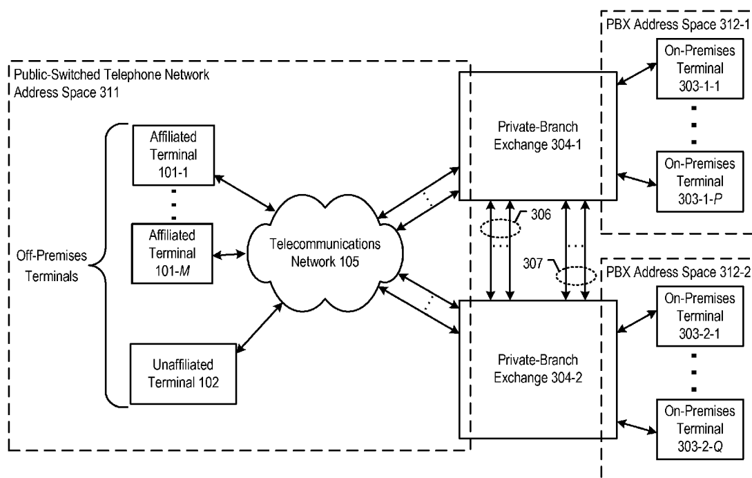
Telecommunications System 300
